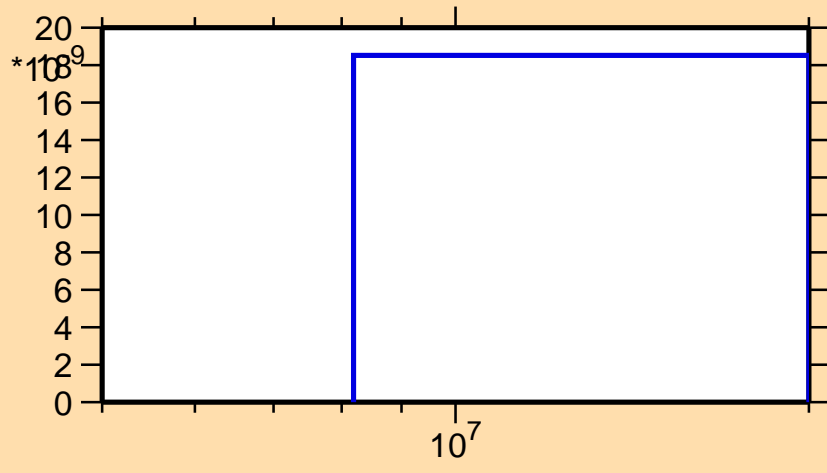
\sigma vs. E for ^{221}\text{Rn}(n,2np)
