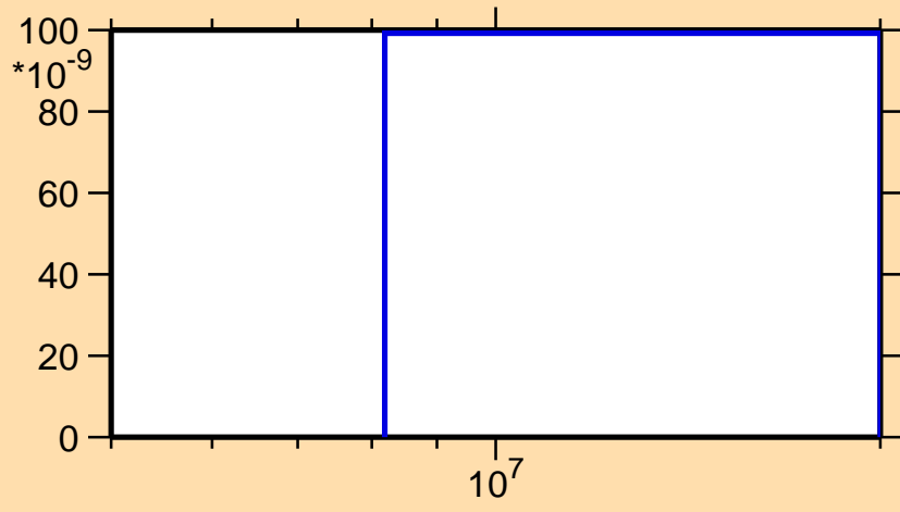
\sigma vs. E for ^{221}\text{Rn}(n,nd)
