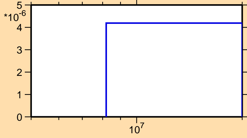
\sigma vs. E for ^{221}\text{Rn} (mt 45)
