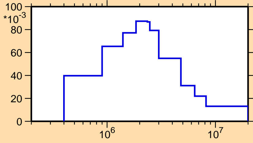
\sigma vs. E for ^{221}\text{Rn}(n,n_3)
