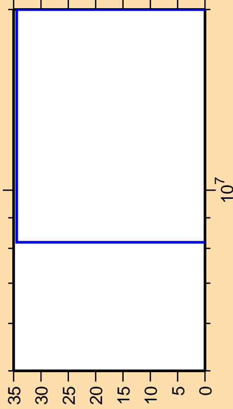
\Delta\sigma/\sigma vs. E for ^{221}\text{Rn} (mt 45)
