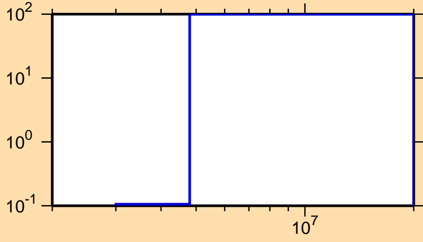
\Delta\sigma/\sigma vs. E for ^{221}\text{Rn}(n,p)
