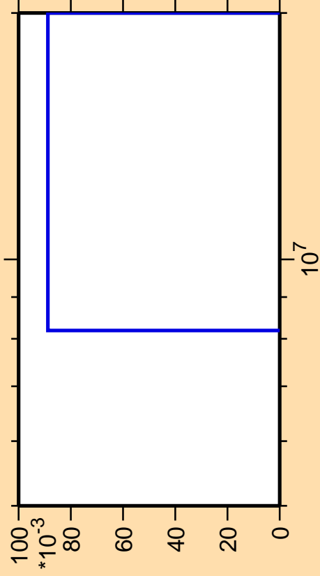
\Delta\sigma/\sigma vs. E for ^{221}\text{Rn}(n,\text{He}3)
