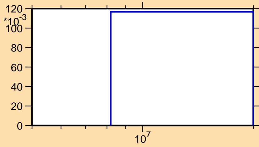
\sigma vs. E for ^{221}\text{Rn}(n,3n\alpha)
