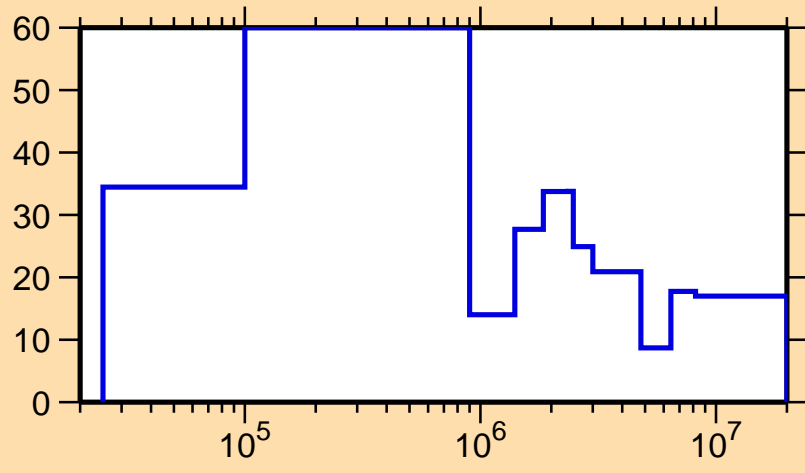
\Delta\sigma/\sigma vs. E for ^{221}\text{Rn}(n,\text{nonel.})
