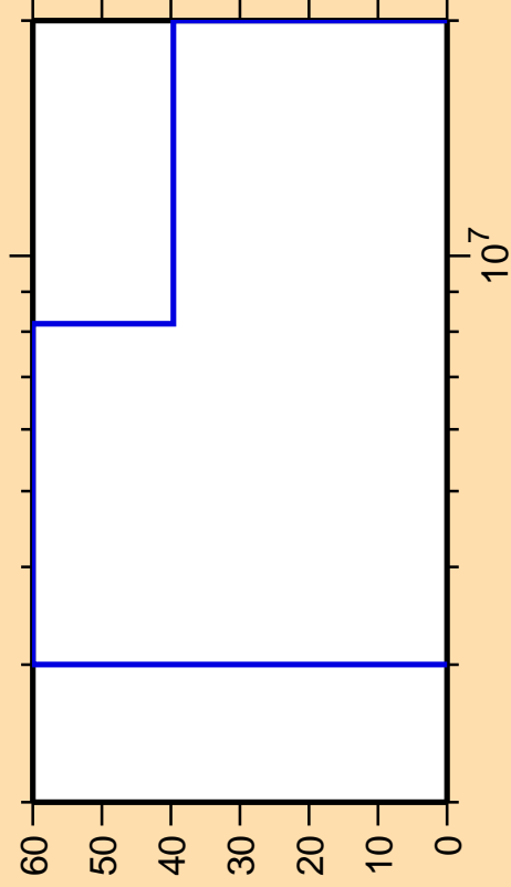
\Delta\sigma/\sigma vs. E for ^{221}\text{Rn}(n,\alpha)
