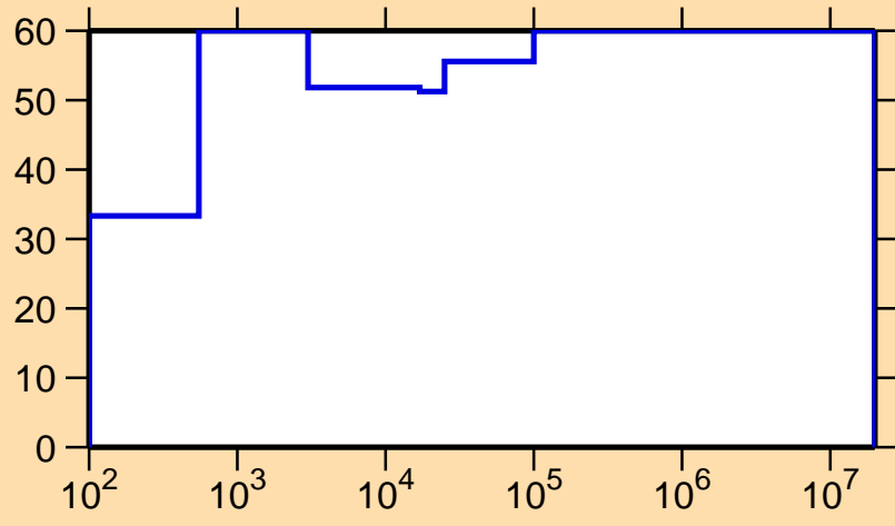
\Delta\sigma/\sigma vs. E for ^{221}\text{Rn}(n,\gamma)
