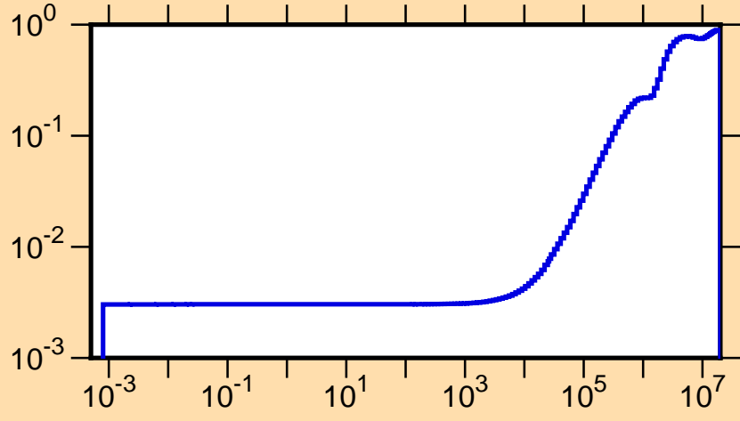
\mu vs. E for ^{222}\text{Rn}(\text{mt251})
