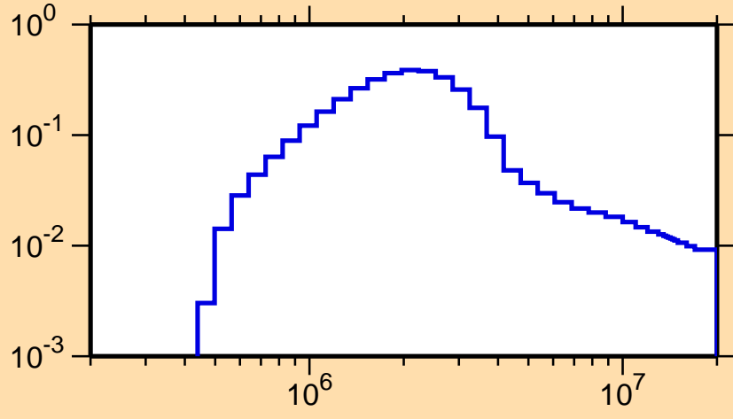
\sigma vs. E for ^{222}\text{Rn}(n,n_2)
