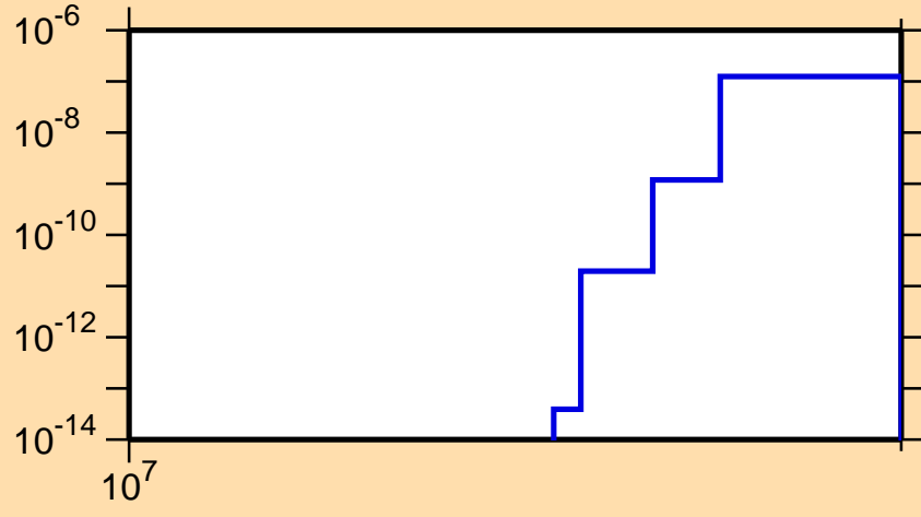
\sigma vs. E for ^{222}\text{Rn}(n,nd)
