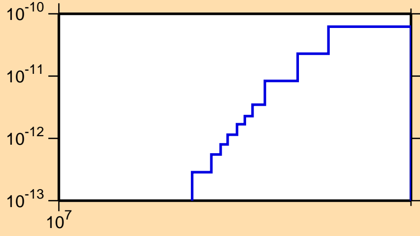
\sigma vs. E for ^{222}\text{Rn}(n,p\alpha)
