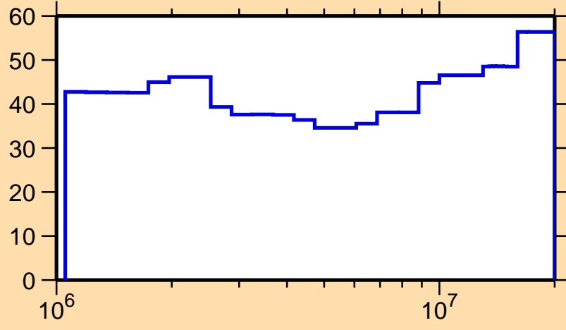
\Delta\sigma/\sigma vs. E for ^{222}\text{Rn}(n,n\text{onel.})
