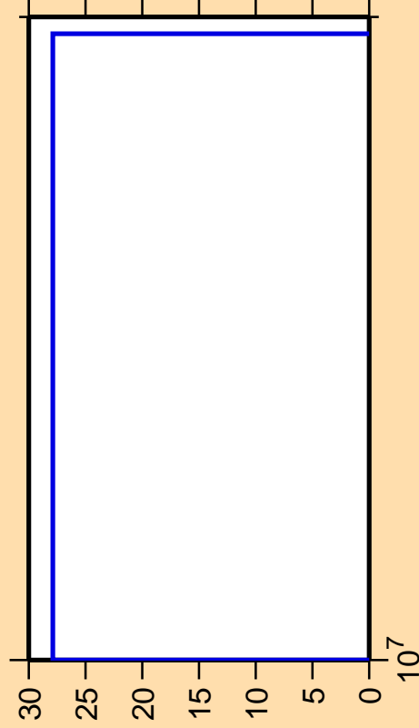
\Delta\sigma/\sigma vs. E for ^{222}\text{Rn}(n,p\alpha)
