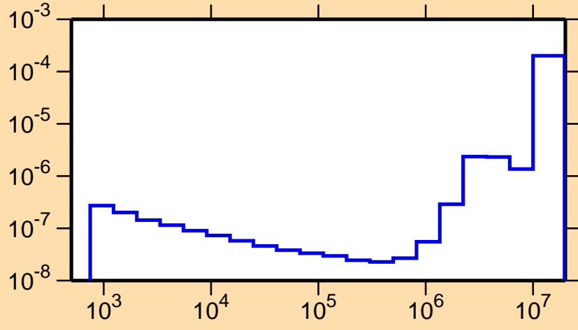
\sigma vs. E for ^{222}\text{Rn}(n,\alpha)
