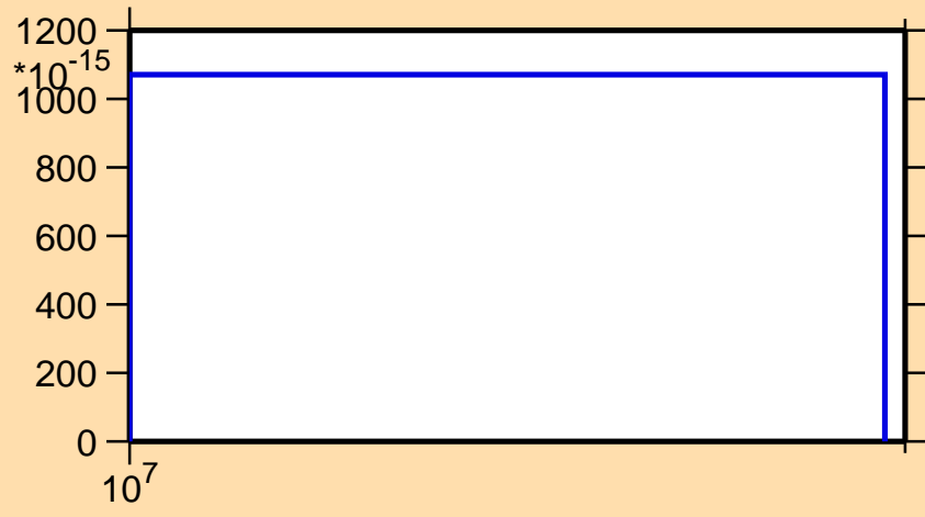
\sigma vs. E for ^{222}\text{Rn} (mt 45)
