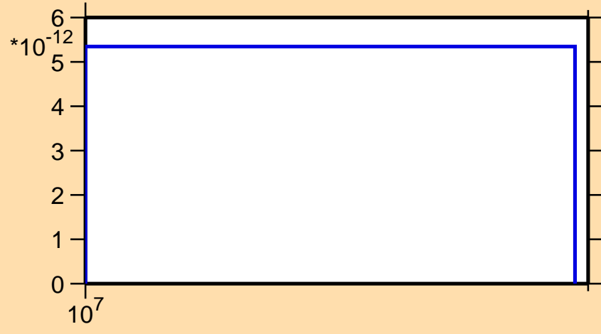
\sigma vs. E for ^{222}\text{Rn}(\text{mt117})
