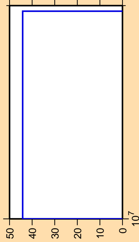
\Delta\sigma/\sigma vs. E for ^{222}\text{Rn}(\text{mt117})
