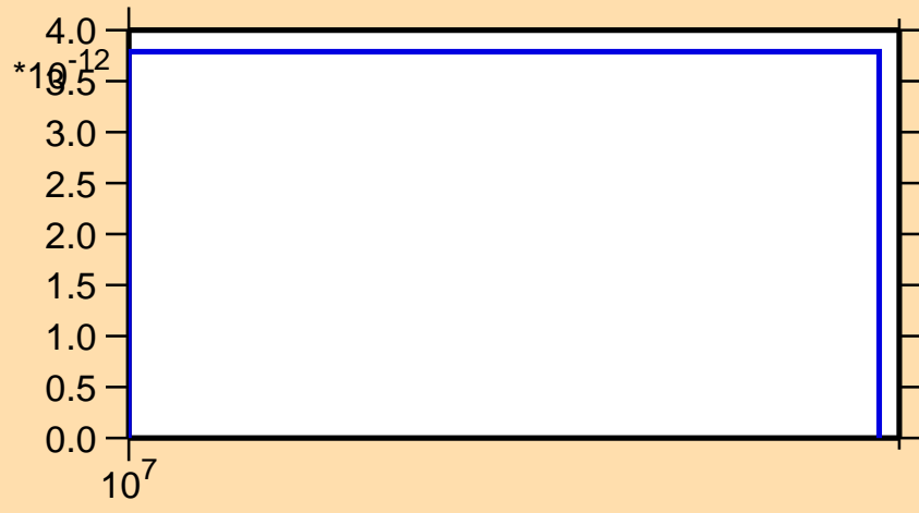
\sigma vs. E for ^{222}\text{Rn}(n,p\alpha)
