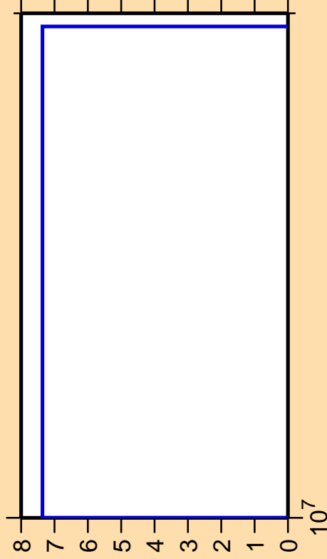
\Delta\sigma/\sigma vs. E for ^{222}\text{Rn} (mt 45)
