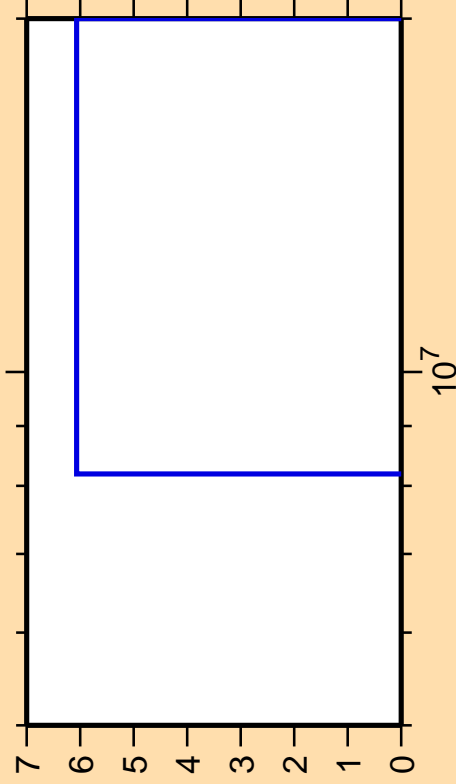
\Delta\sigma/\sigma vs. E for ^{222}\text{Rn} (mt 45)
