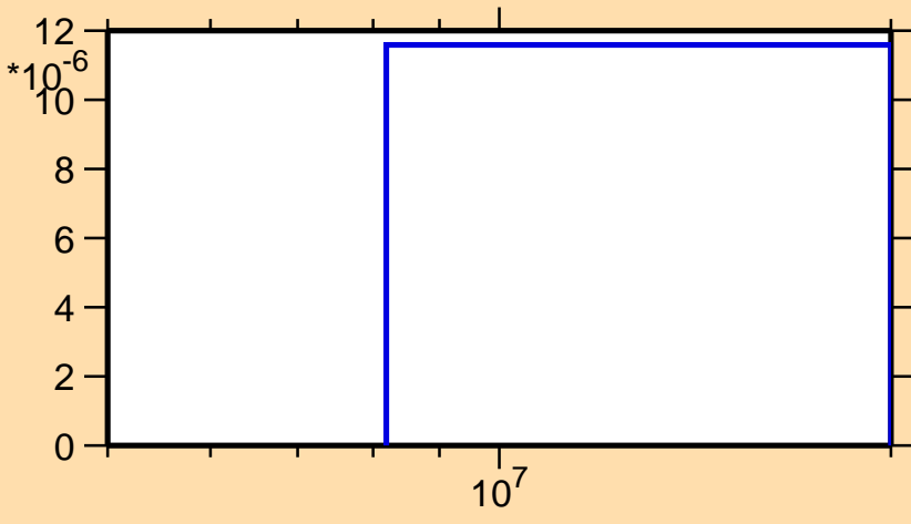
\sigma vs. E for ^{222}\text{Rn}(n,np)
