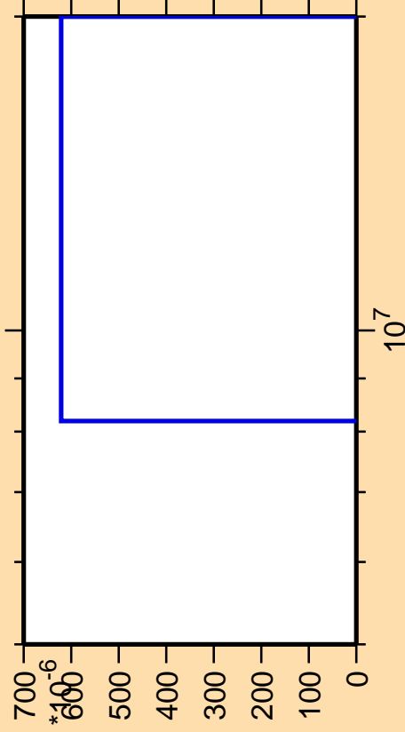
\Delta\sigma/\sigma vs. E for ^{222}\text{Rn}(\text{mt 11})
