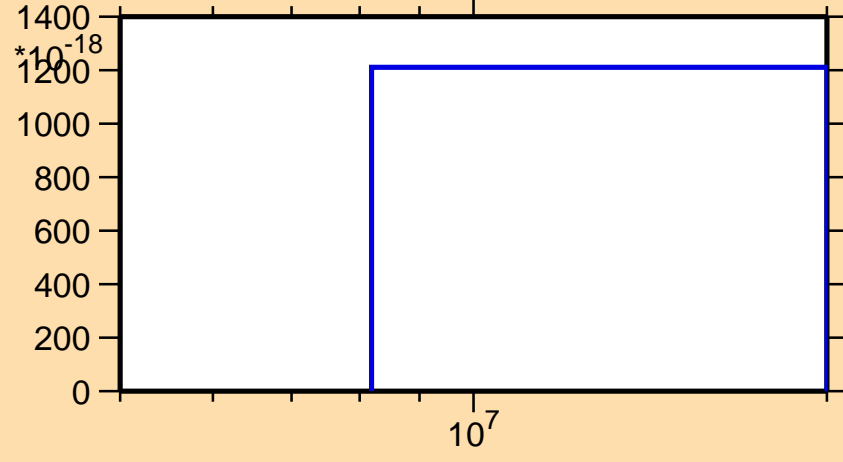
\sigma vs. E for ^{222}\text{Rn}(\text{mt 11})
