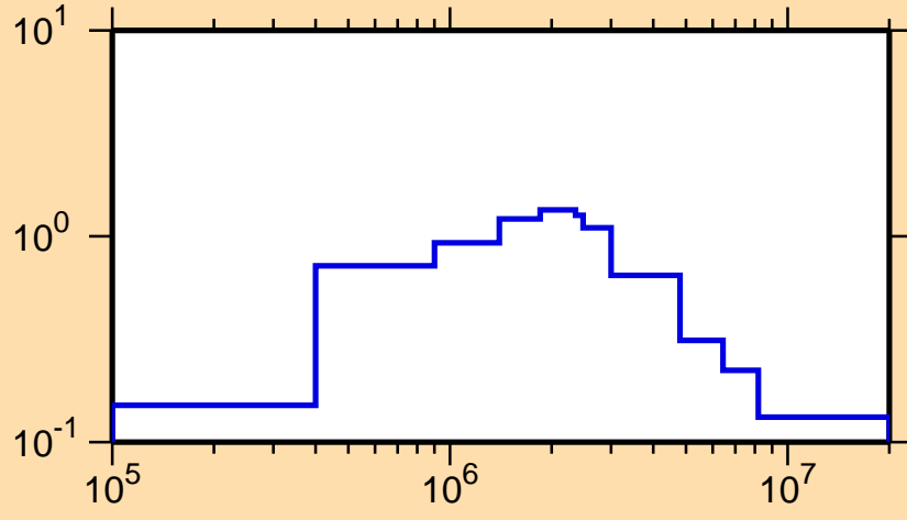
\sigma vs. E for ^{222}\text{Rn}(n,n_1)
