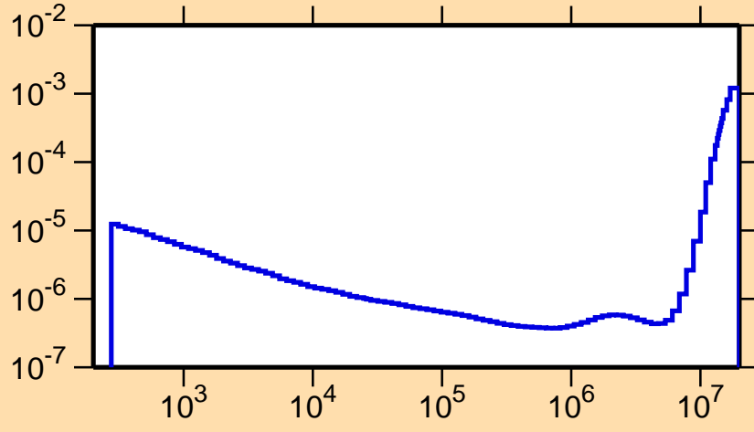
\sigma vs. E for ^{223}\text{Rn}(n,\alpha)
