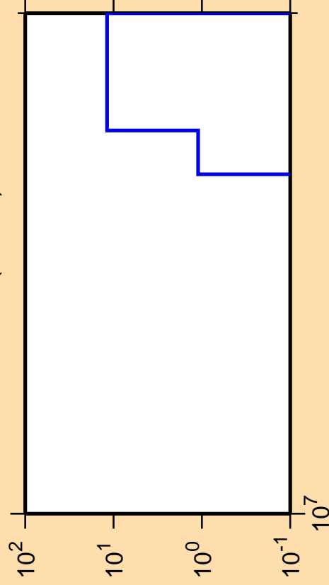
\Delta\sigma/\sigma vs. E for ^{223}\text{Rn} (mt 45)
