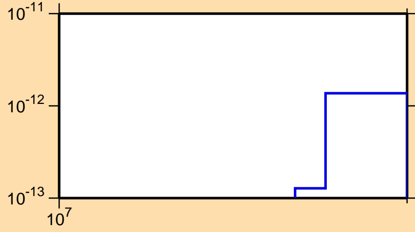
\sigma vs. E for ^{223}\text{Rn} (mt 45)
