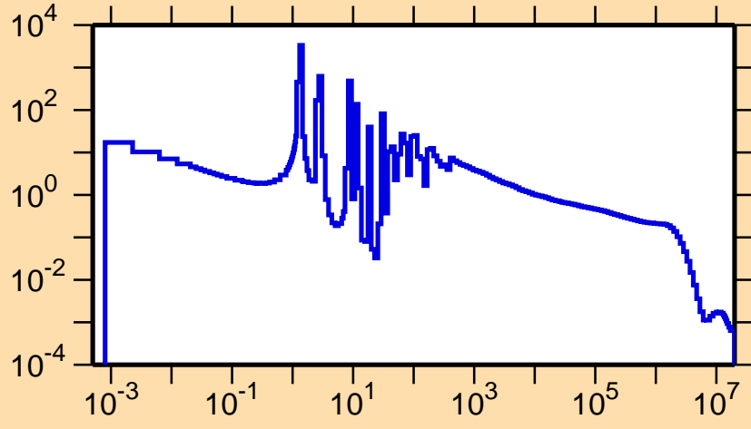
\sigma vs. E for ^{223}\text{Rn}(n,\gamma)
