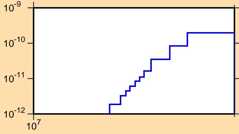
\sigma vs. E for ^{223}\text{Rn}(n,p\alpha)
