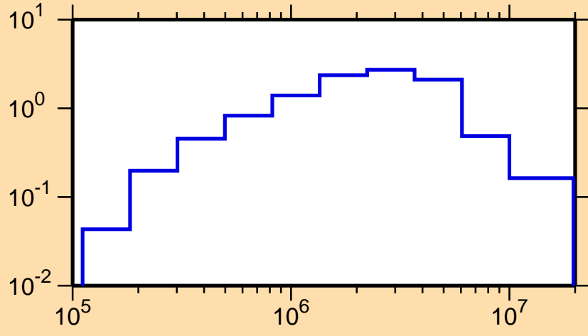
\sigma vs. E for ^{223}\text{Rn}(n,\text{inel.})
