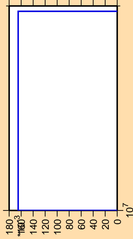
\Delta\sigma/\sigma vs. E for ^{223}\text{Rn} (mt 45)
