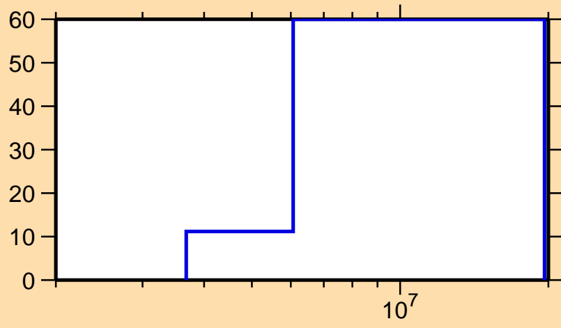
\Delta\sigma/\sigma vs. E for ^{223}\text{Rn}(n,p)
