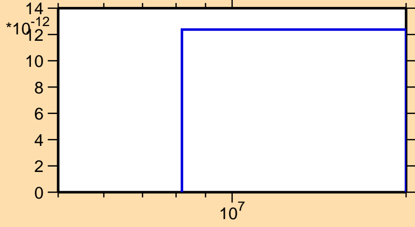
\sigma vs. E for ^{223}\text{Rn}(n,p\alpha)
