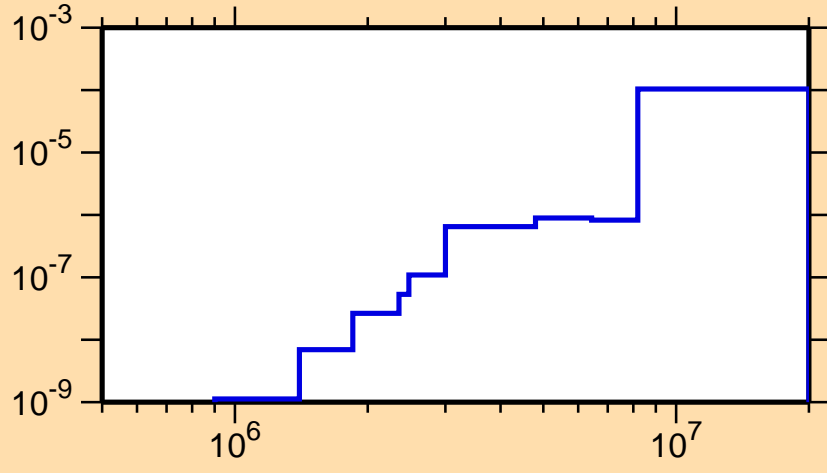
\sigma vs. E for ^{223}\text{Rn}(n,n\alpha)
