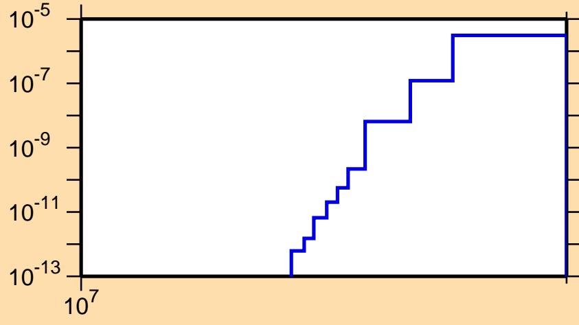
\sigma vs. E for ^{224}\text{Rn}(n,nt)
