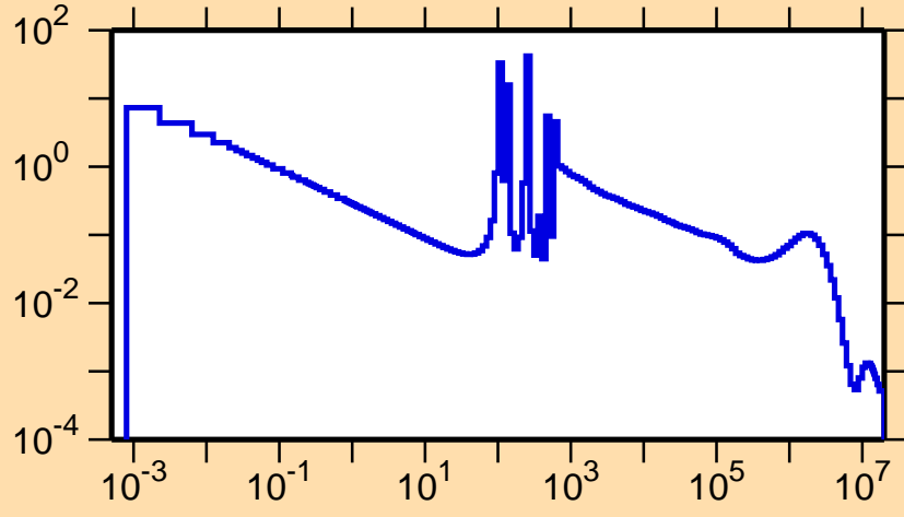
\sigma vs. E for ^{224}\text{Rn}(n,\gamma)
