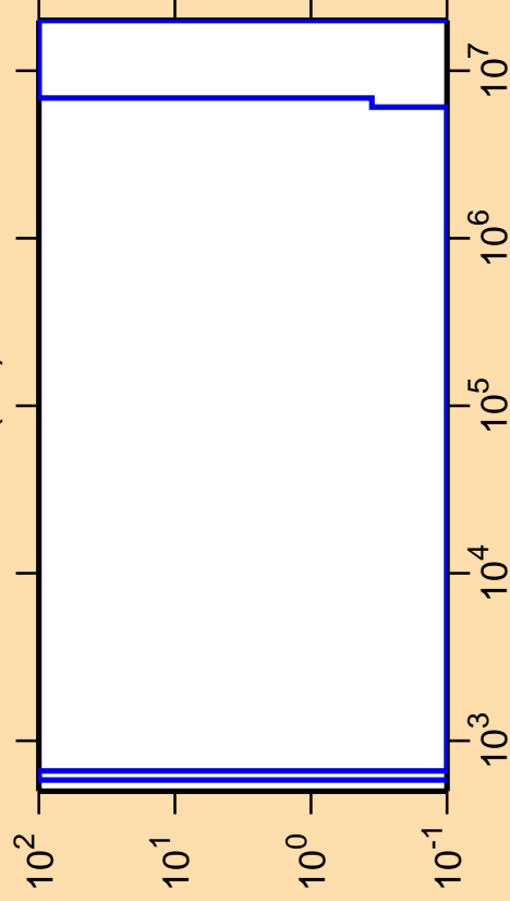
\Delta\sigma/\sigma vs. E for ^{224}\text{Rn}(n,f)
