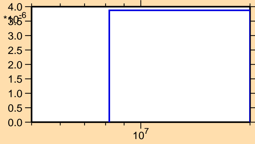
\sigma vs. E for ^{224}\text{Rn}(n,np)
