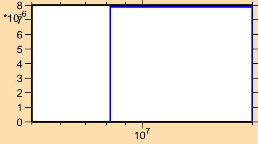
\sigma vs. E for ^{224}\text{Rn}(n,t)
