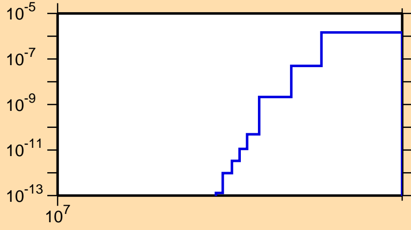
\sigma vs. E for ^{225}\text{Rn}(n,\text{nd})
