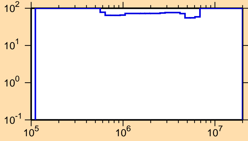
\Delta\sigma/\sigma vs. E for ^{225}\text{Rn}(n,n\text{cont.})
