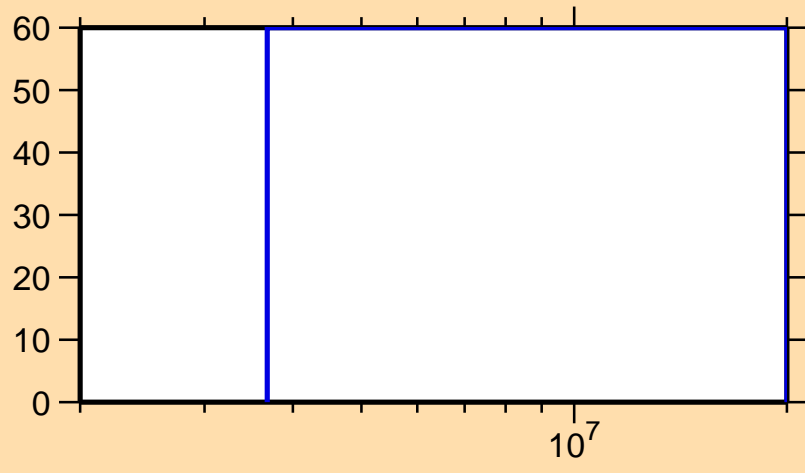
\Delta\sigma/\sigma vs. E for ^{225}\text{Rn}(n,2n)
