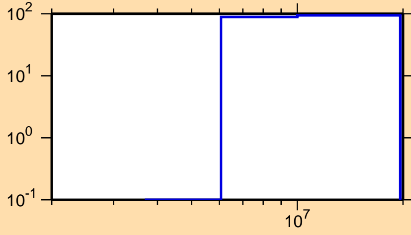
\Delta\sigma/\sigma vs. E for ^{225}\text{Rn}(n,p)
