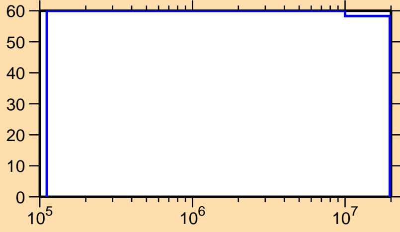
\Delta\sigma/\sigma vs. E for ^{225}\text{Rn}(n,n_1)
