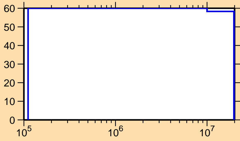
\Delta\sigma/\sigma vs. E for ^{225}\text{Rn}(n,n_1)
