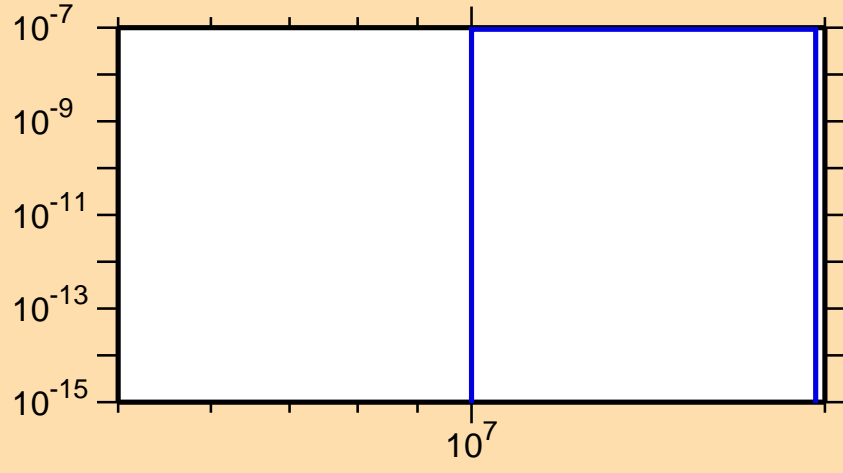
\sigma vs. E for ^{225}\text{Rn}(n,3n\alpha)
