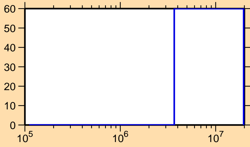
\Delta\sigma/\sigma vs. E for ^{225}\text{Rn}(n,f)
