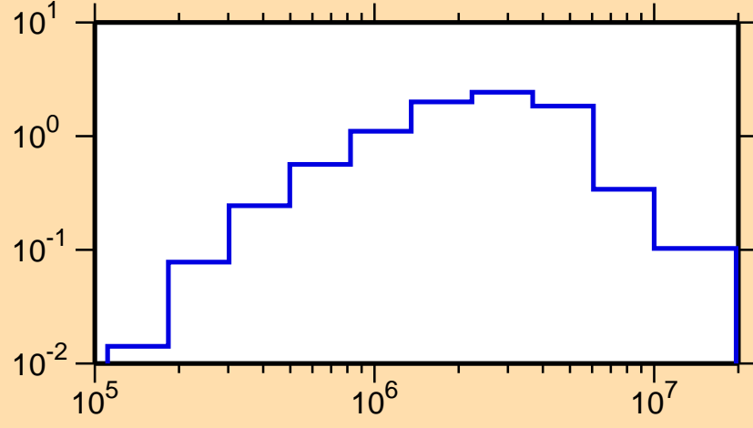
\sigma vs. E for ^{225}\text{Rn}(n,n\text{cont.})
