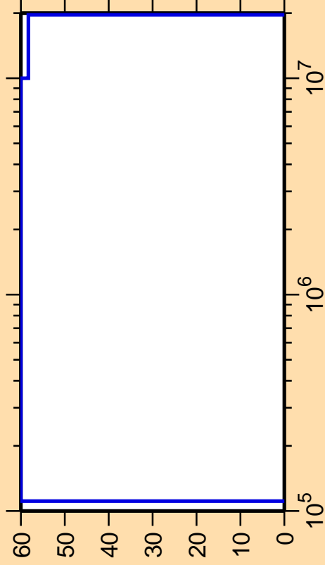
\Delta\sigma/\sigma vs. E for ^{225}\text{Rn}(n,n_1)
