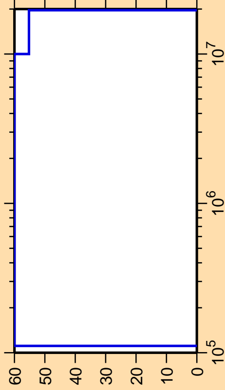
\Delta\sigma/\sigma vs. E for ^{225}\text{Rn}(n,\alpha)
