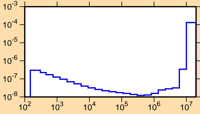
\sigma vs. E for ^{225}\text{Rn}(n,\alpha)
