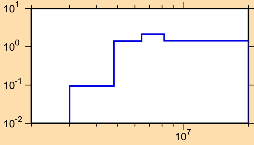
\sigma vs. E for ^{225}\text{Rn}(n,2n)
