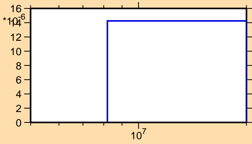
\sigma vs. E for ^{225}\text{Rn}(n,d)
