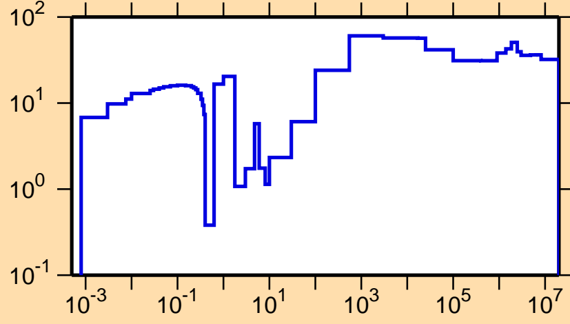
\Delta\sigma/\sigma vs. E for ^{225}\text{Rn}(n,tot.)
