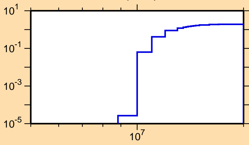
\sigma vs. E for ^{226}\text{Rn}(n,3n)
