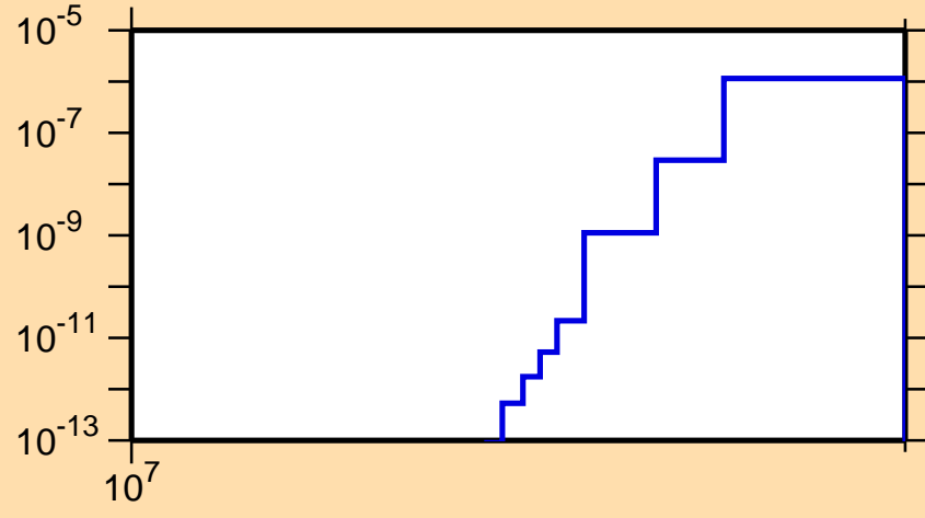
\sigma vs. E for ^{226}\text{Rn}(n,nt)
