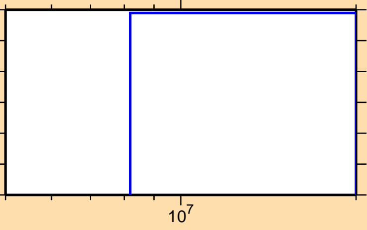
\sigma vs. E for ^{226}\text{Rn}(n,3n\alpha)
