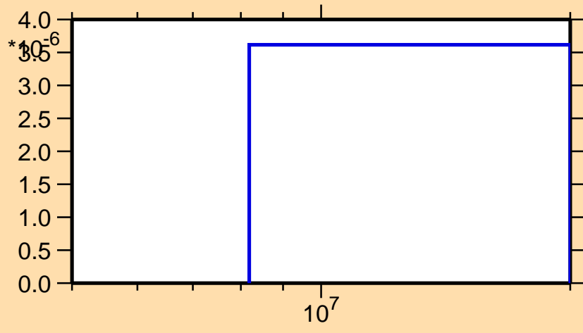
\sigma vs. E for ^{226}\text{Rn}(n,t)
