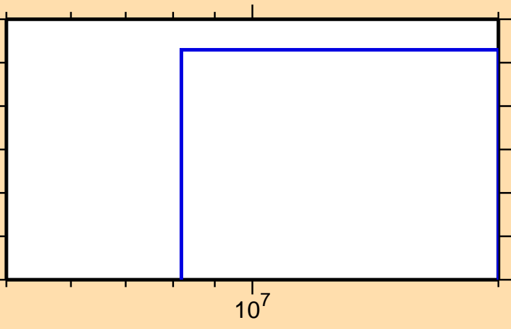
\sigma vs. E for ^{226}\text{Rn}(n,2np)
