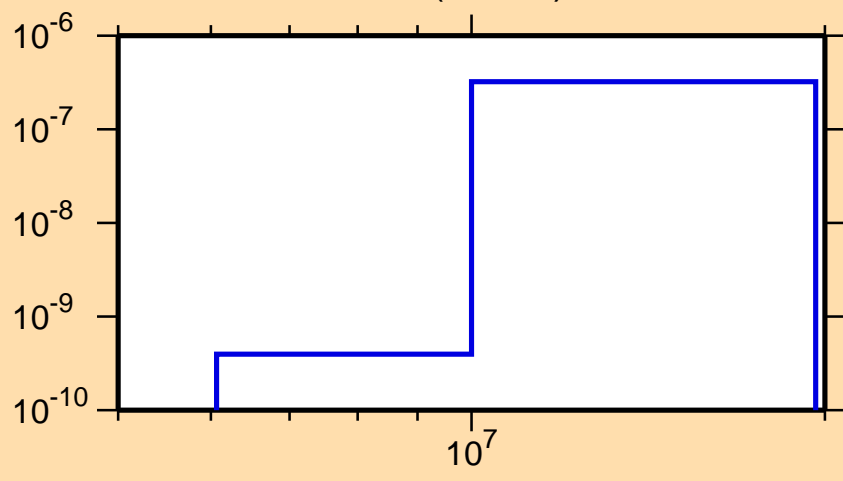
\sigma vs. E for ^{227}\text{Rn}(n,2n\alpha)
