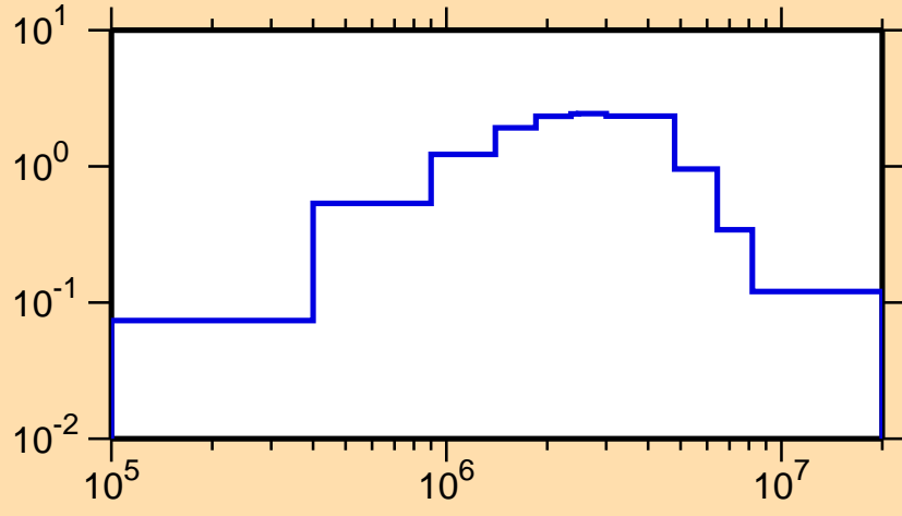
\sigma vs. E for ^{227}\text{Rn}(n,n\text{cont.})
