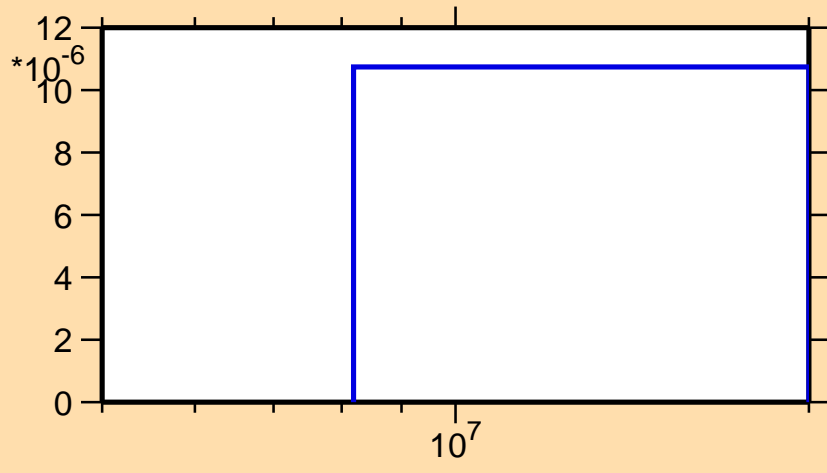
\sigma vs. E for ^{227}\text{Rn}(n,t)
