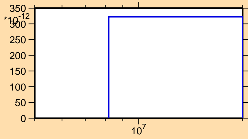
\sigma vs. E for ^{227}\text{Rn}(n,2np)
