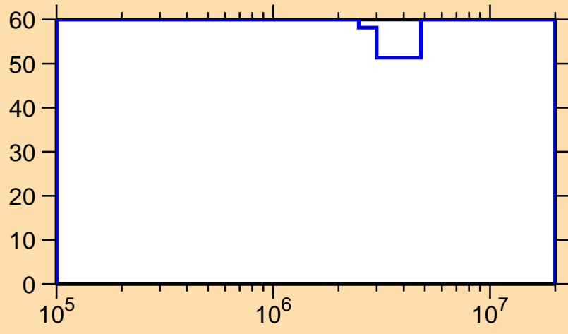
\Delta\sigma/\sigma vs. E for ^{227}\text{Rn}(n,n_1)
