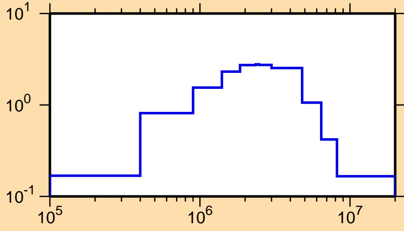
\sigma vs. E for ^{227}\text{Rn}(n,\text{inel.})
