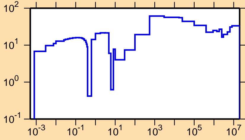
\Delta\sigma/\sigma vs. E for ^{227}\text{Rn}(n,tot.)
