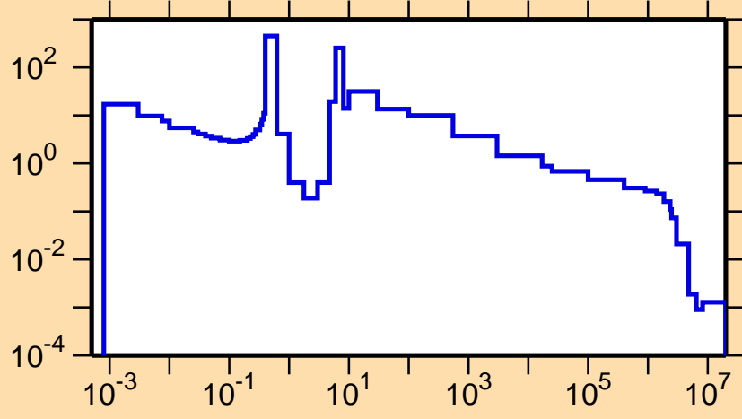
\sigma vs. E for ^{227}\text{Rn}(n,\gamma)
