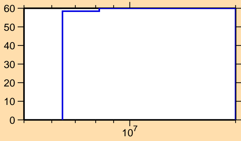
\Delta\sigma/\sigma vs. E for ^{227}\text{Rn}(n,p)
