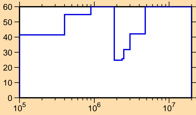
\Delta\sigma/\sigma vs. E for ^{227}\text{Rn}(n,\text{el.})
