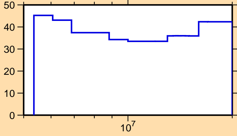
\Delta\sigma/\sigma vs. E for ^{228}\text{Rn}(n,\text{tot.})
