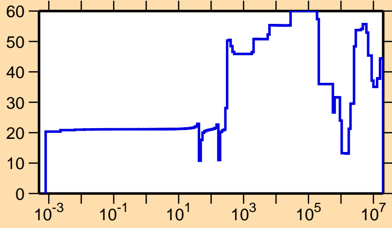
\Delta\sigma/\sigma vs. E for ^{228}\text{Rn}(n,\text{el.})
