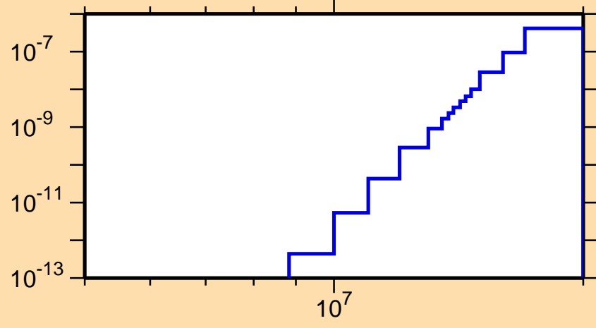
\sigma vs. E for ^{228}\text{Rn}(n,2n\alpha)
