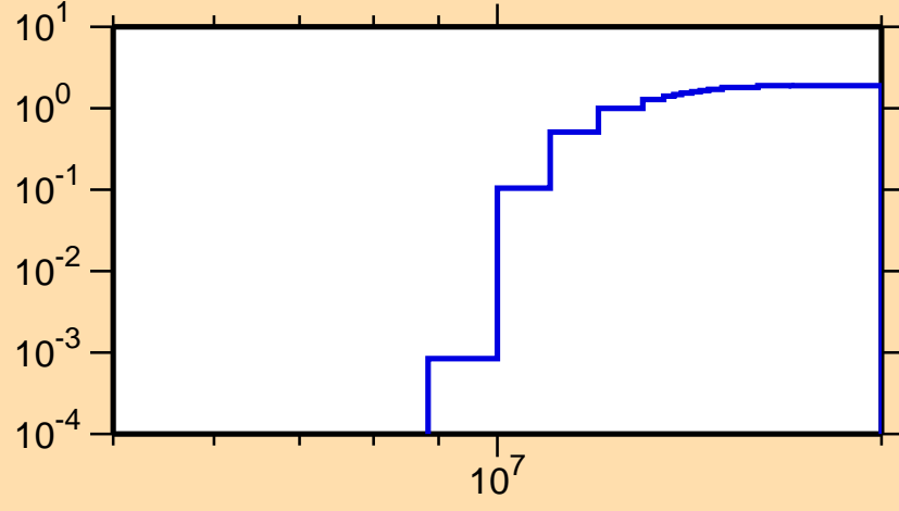
\sigma vs. E for ^{228}\text{Rn}(n,3n)
