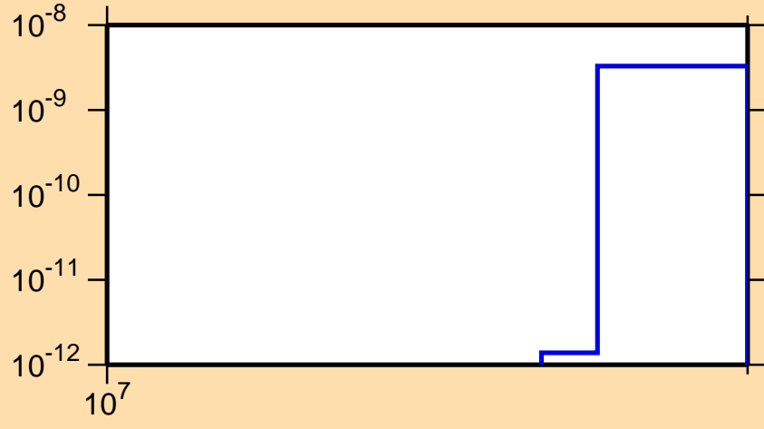
\sigma vs. E for ^{228}\text{Rn}(n,nd)
