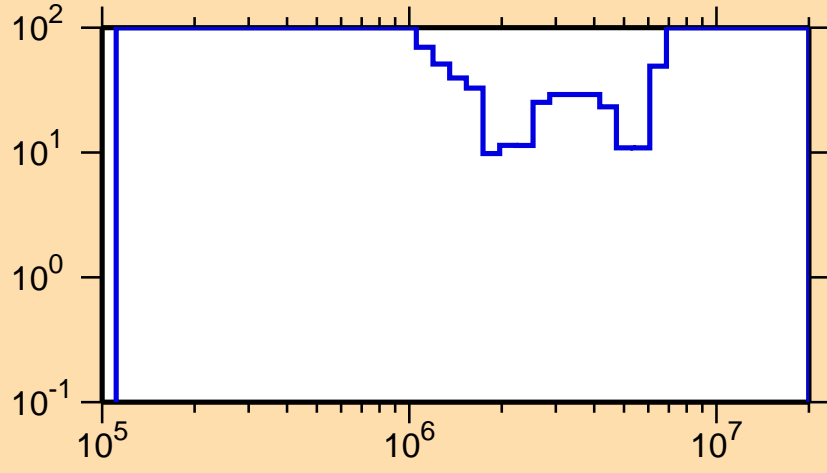
\Delta\sigma/\sigma vs. E for ^{228}\text{Rn}(n,n\text{cont.})
