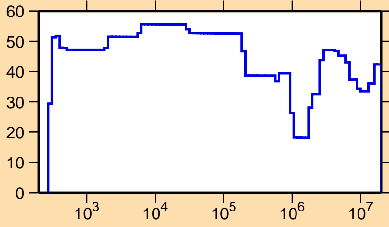
\Delta\sigma/\sigma vs. E for ^{228}\text{Rn}(n,\text{tot.})
