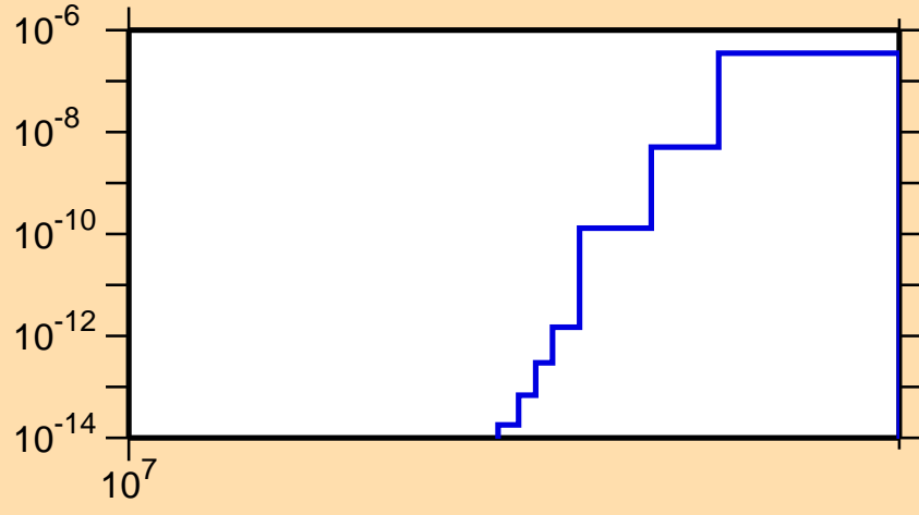
\sigma vs. E for ^{228}\text{Rn}(n,nt)
