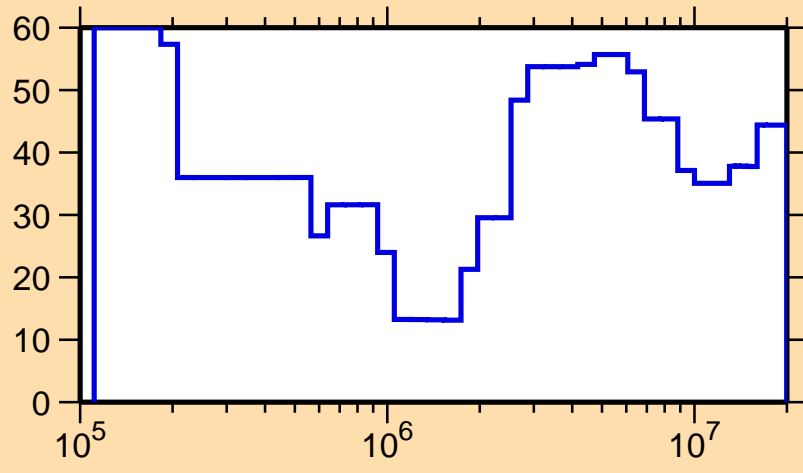
\Delta\sigma/\sigma vs. E for ^{228}\text{Rn}(n,\text{el.})
