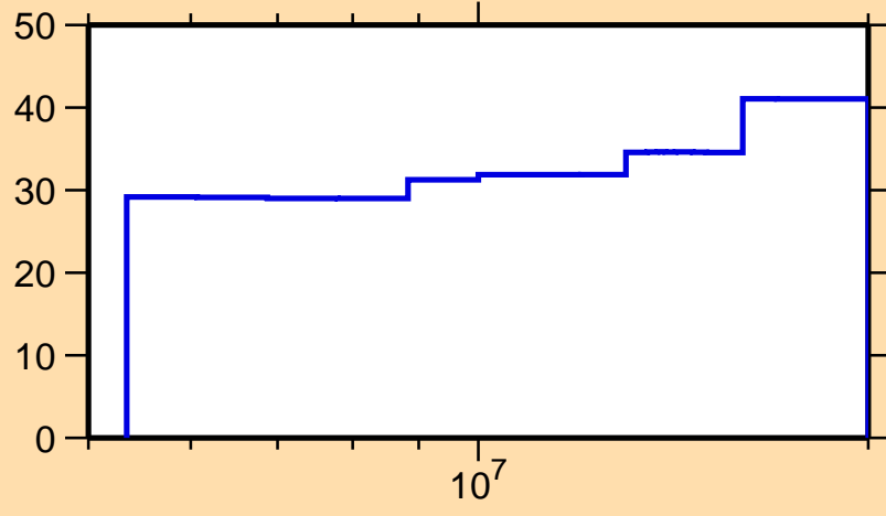
\Delta\sigma/\sigma vs. E for ^{228}\text{Rn}(n,\text{nonel.})
