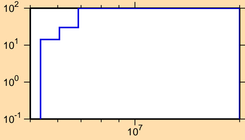
\Delta\sigma/\sigma vs. E for ^{228}\text{Rn}(n,\text{inel.})
