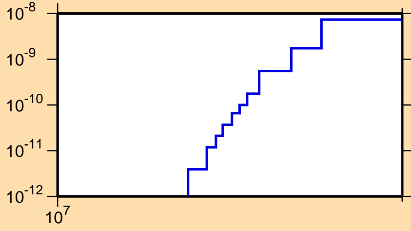
\sigma vs. E for ^{228}\text{Rn}(n,3n\alpha)
