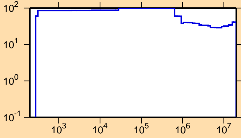
\Delta\sigma/\sigma vs. E for ^{228}\text{Rn}(n,\text{nonel.})
