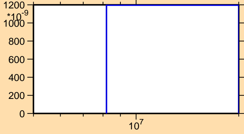
\sigma vs. E for ^{228}\text{Rn}(n,d)
