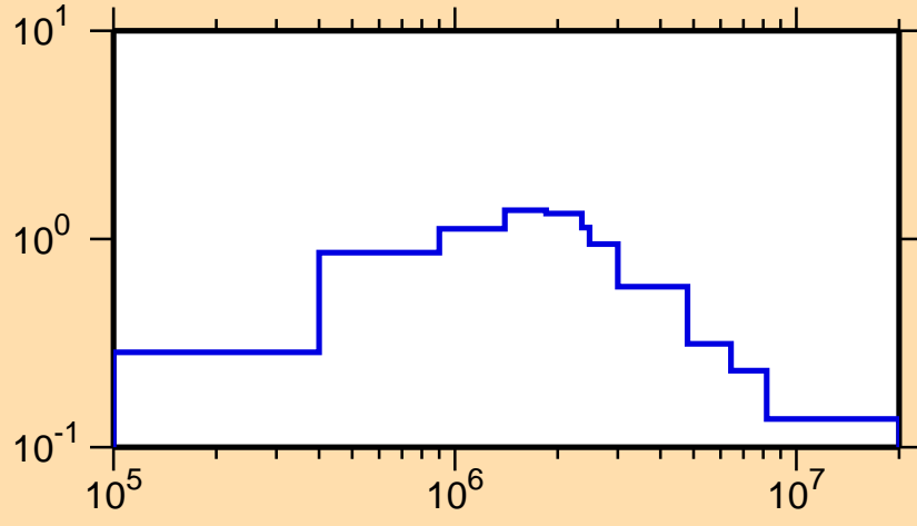
\sigma vs. E for ^{228}\text{Rn}(n,n_1)
