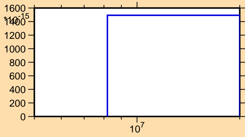
\sigma vs. E for ^{228}\text{Rn}(n,2np)
