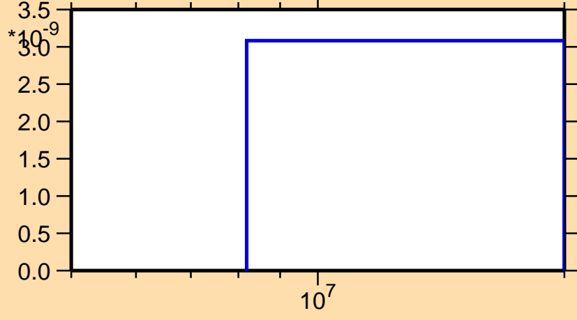
\sigma vs. E for ^{228}\text{Rn}(n,nt)
