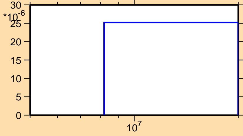
\sigma vs. E for ^{228}\text{Rn}(n,p)
