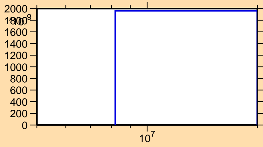
\sigma vs. E for ^{228}\text{Rn}(n,t)
