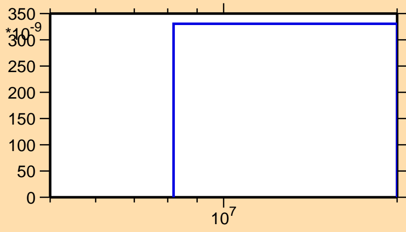
\sigma vs. E for ^{228}\text{Rn}(n,np)
