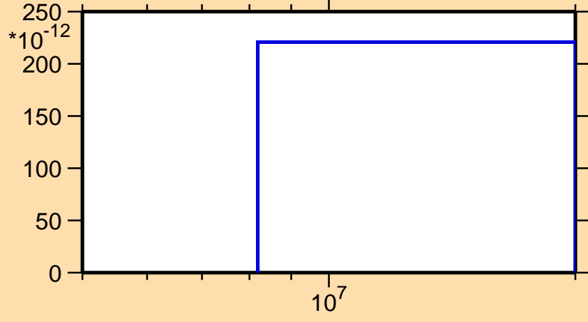
\sigma vs. E for ^{228}\text{Rn}(n,3n\alpha)
