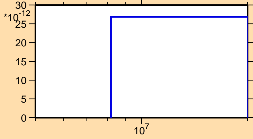
\sigma vs. E for ^{228}\text{Rn}(n,\text{nd})
