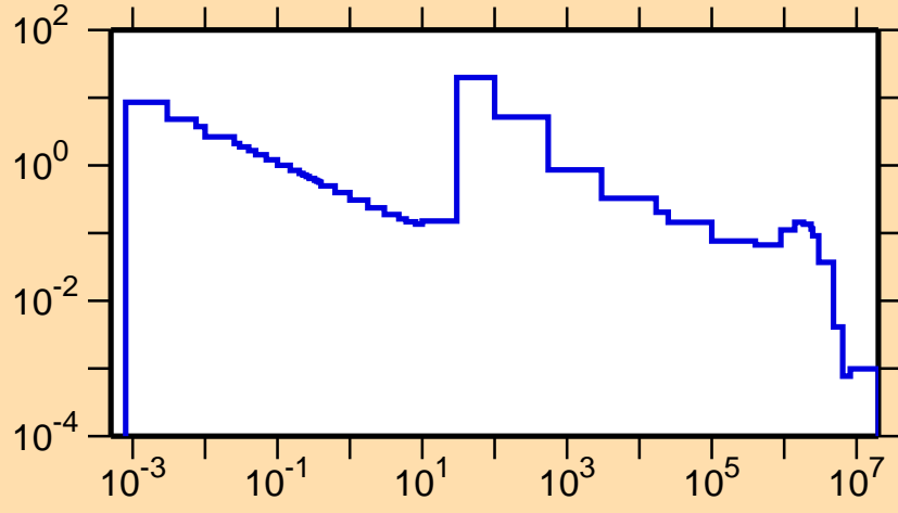
\sigma vs. E for ^{228}\text{Rn}(n,\gamma)
