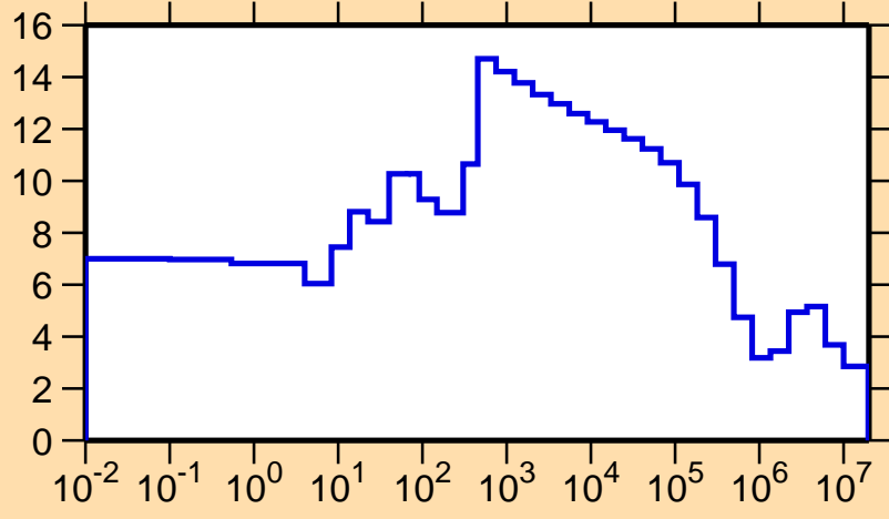
\sigma vs. E for ^{229}\text{Rn}(n,\text{el.})
