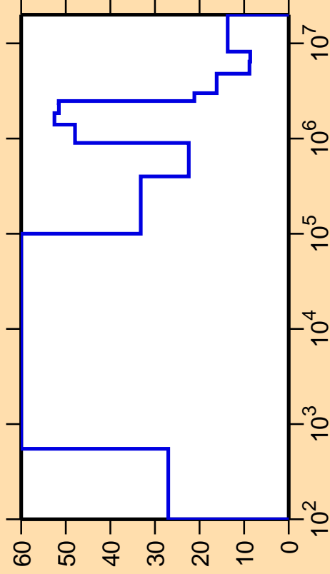
\Delta\sigma/\sigma vs. E for ^{229}\text{Rn}(n,\text{nonel.})
