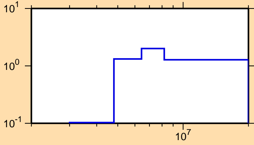
\sigma vs. E for ^{229}\text{Rn}(n,2n)
