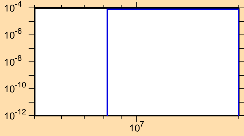
\sigma vs. E for ^{229}\text{Rn}(n,p)
