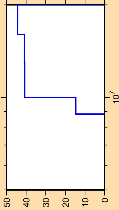
\Delta\sigma/\sigma vs. E for ^{230}\text{Rn}(n,p)
