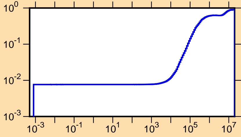
\mu vs. E for ^{88}\text{Ru}(\text{mt251})
