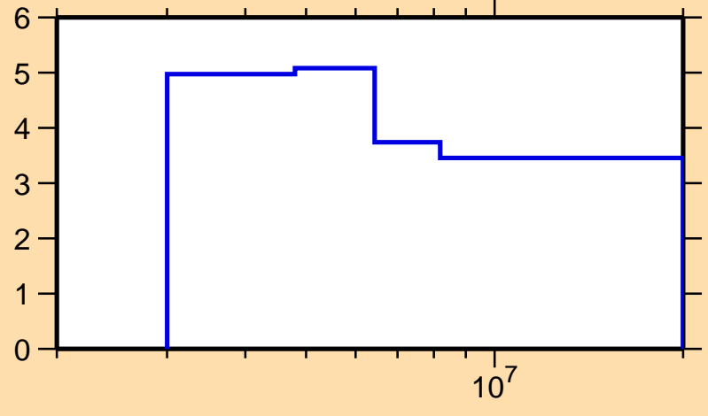
\Delta\sigma/\sigma vs. E for ^{88}\text{Ru}(n,n\text{onel.})
