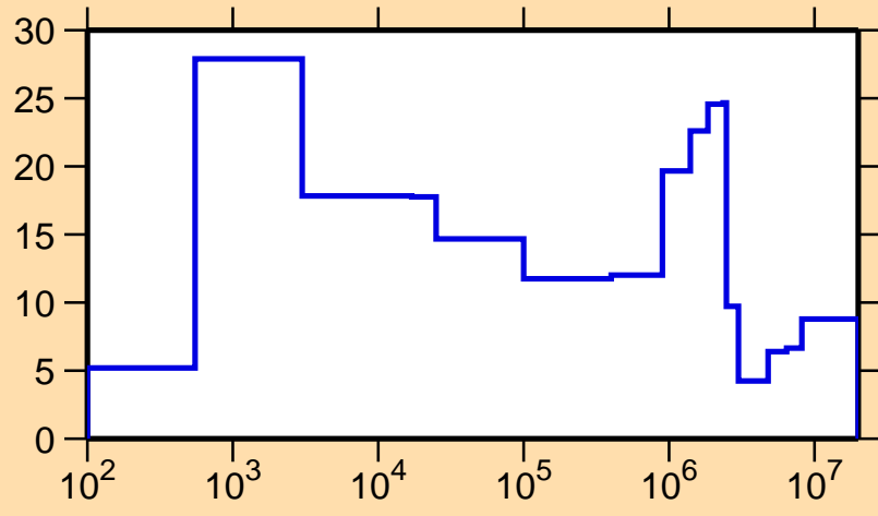
\Delta\sigma/\sigma vs. E for ^{88}\text{Ru}(n,el.)
