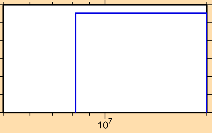
\sigma vs. E for ^{89}\text{Ru}(n,2n)
