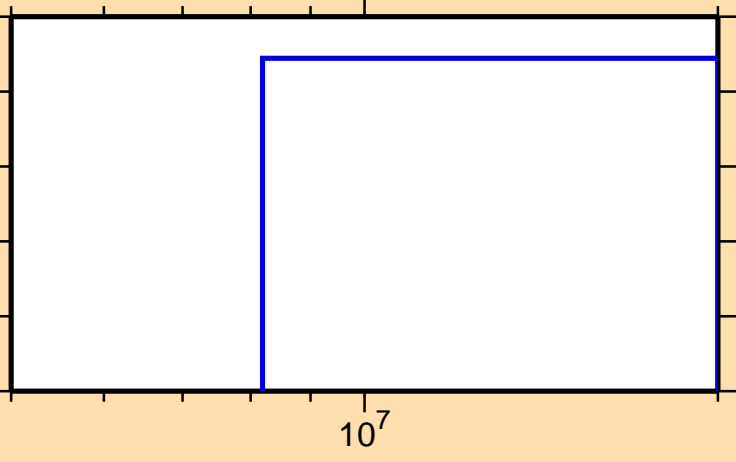
\sigma vs. E for ^{89}\text{Ru}(n,2np)
