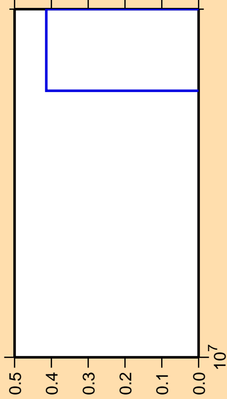
\Delta\sigma/\sigma vs. E for ^{90}\text{Ru}(n,2np)
