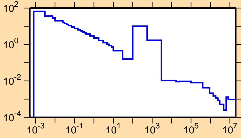
\sigma vs. E for ^{90}\text{Ru}(n,\gamma)
