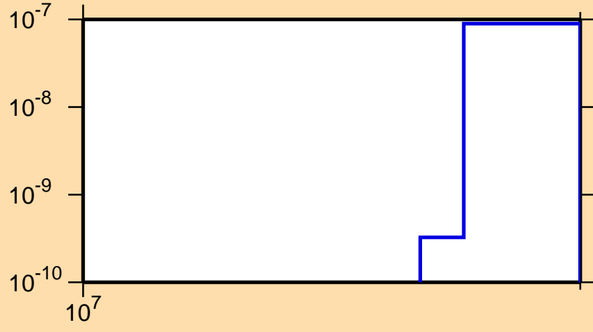
\sigma vs. E for ^{91}\text{Ru}(n,\text{nd})
