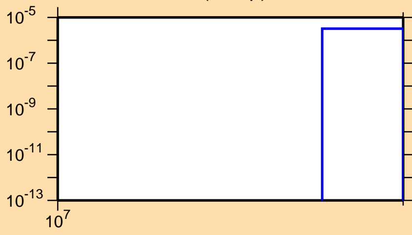
\sigma vs. E for ^{91}\text{Ru}(n,2np)
