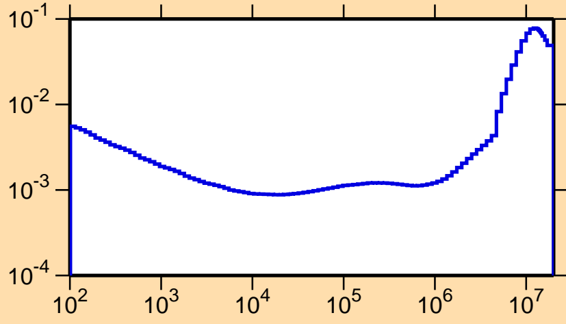
\sigma vs. E for ^{91}\text{Ru}(n,\alpha)
