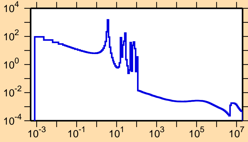
\sigma vs. E for ^{91}\text{Ru}(n,\gamma)
