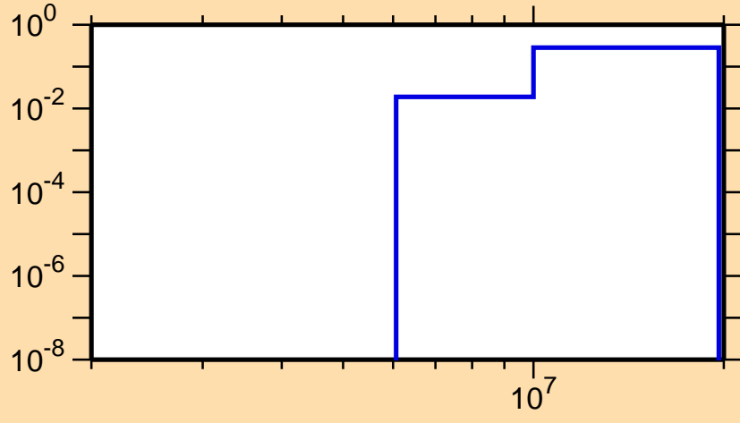
\sigma vs. E for ^{91}\text{Ru}(n,np)
