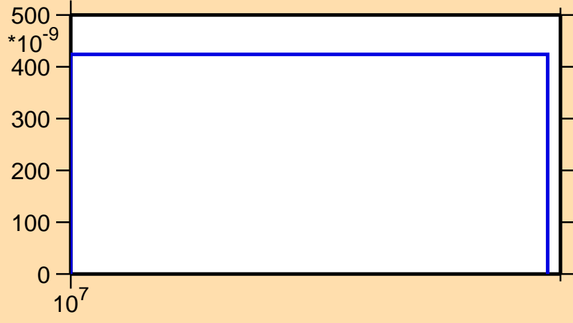
\sigma vs. E for ^{91}\text{Ru}(n,\text{pt})
