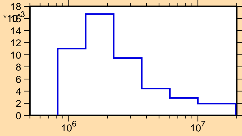
\sigma vs. E for ^{91}\text{Ru}(n,n_3)
