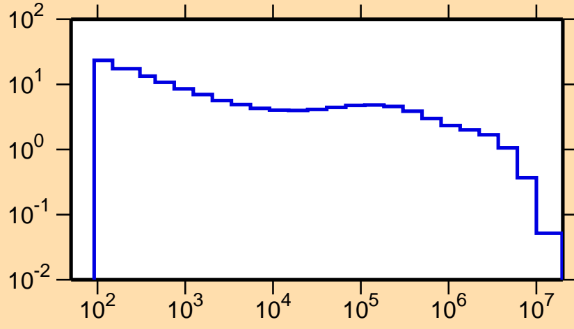
\sigma vs. E for ^{91}\text{Ru}(n,p)
