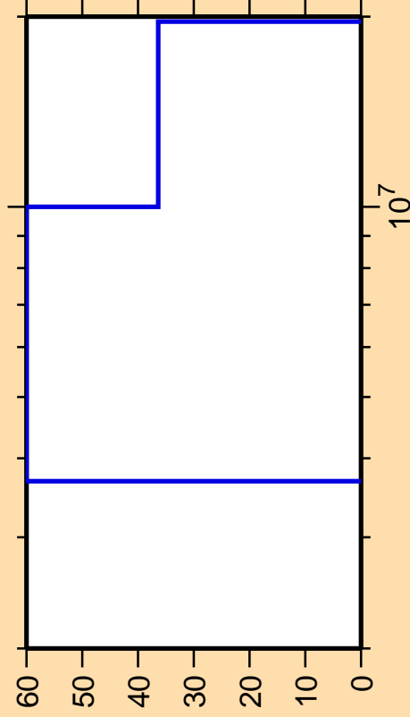
\Delta\sigma/\sigma vs. E for ^{91}\text{Ru}(n,np)
