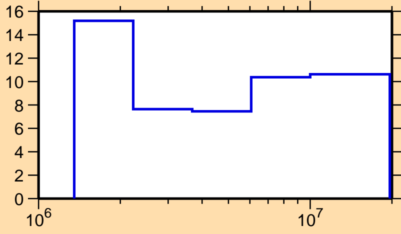
\Delta\sigma/\sigma vs. E for ^{91}\text{Ru}(n,n\text{nonel.})
