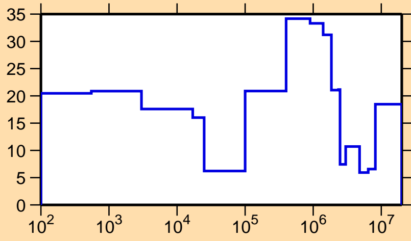
\Delta\sigma/\sigma vs. E for ^{91}\text{Ru}(n,\text{el.})
