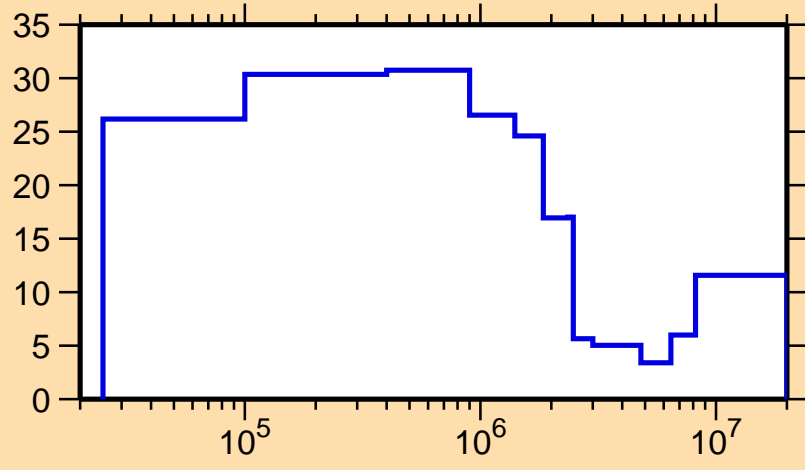
\Delta\sigma/\sigma vs. E for ^{91}\text{Ru}(n,\text{tot.})
