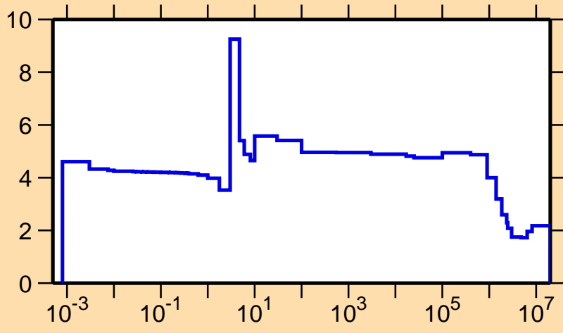
\sigma vs. E for ^{91}\text{Ru}(n,\text{el.})
