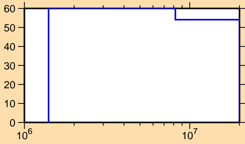
\Delta\sigma/\sigma vs. E for ^{91}\text{Ru}(n,n\text{cont.})
