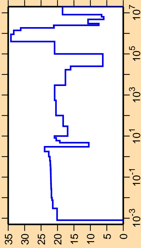
\Delta\sigma/\sigma vs. E for ^{91}\text{Ru}(n,\text{el.})
