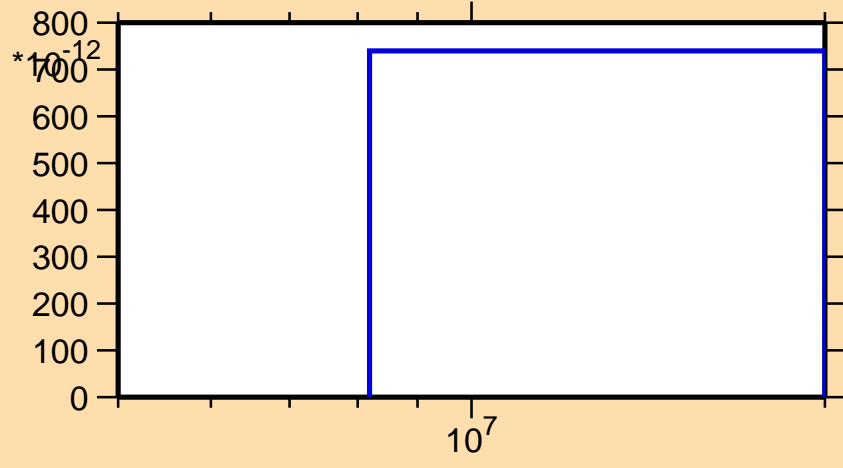
\sigma vs. E for ^{91}\text{Ru}(n,\text{nd})
