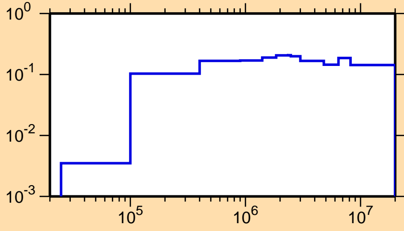
\sigma vs. E for ^{91}\text{Ru}(n,\text{inel.})
