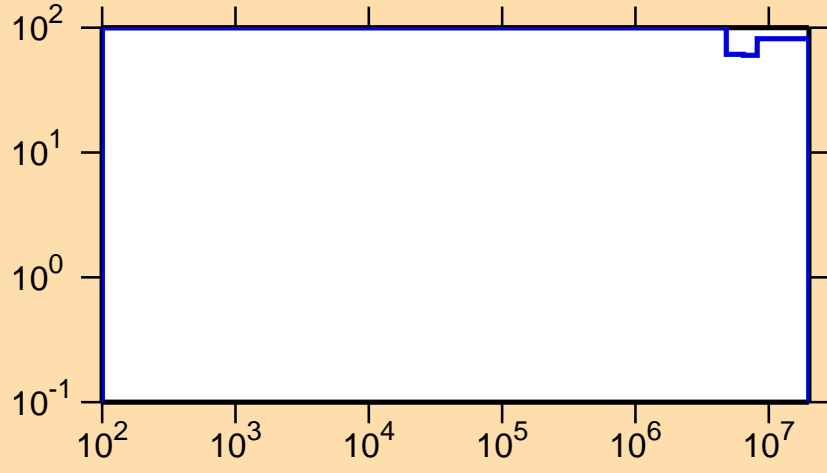
\Delta\sigma/\sigma vs. E for ^{91}\text{Ru}(n,\gamma)
