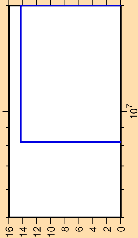
\Delta\sigma/\sigma vs. E for ^{91}\text{Ru}(\text{mt117})
