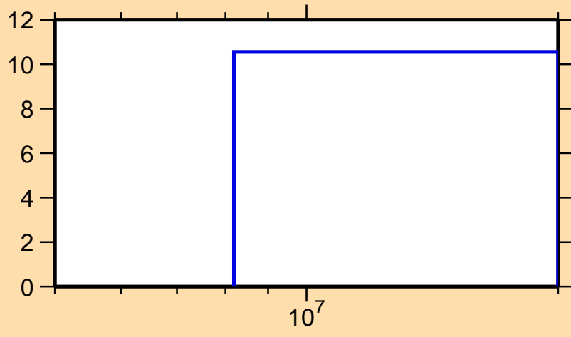
\Delta\sigma/\sigma vs. E for ^{91}\text{Ru}(n,\text{nonel.})
