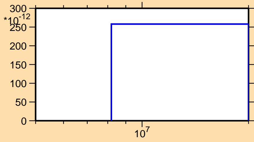
\sigma vs. E for ^{91}\text{Ru} (mt 45)
