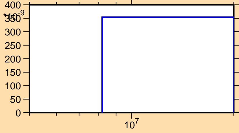
\sigma vs. E for ^{91}\text{Ru}(n,\text{pt})
