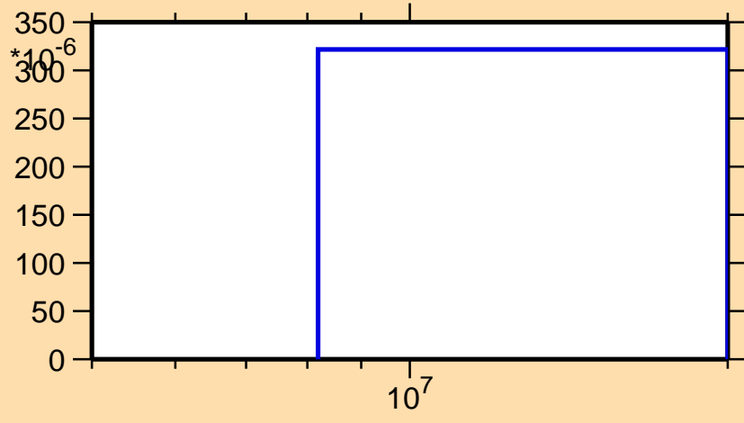
\sigma vs. E for ^{91}\text{Ru}(n,2n)
