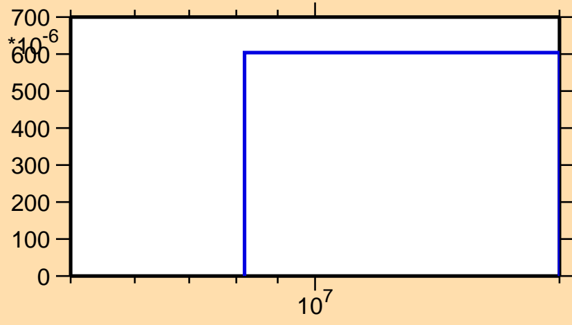
\sigma vs. E for ^{91}\text{Ru}(n,\text{pd})
