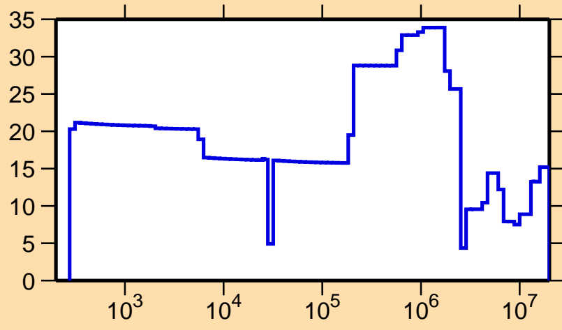
\Delta\sigma/\sigma vs. E for ^{93}\text{Ru}(n,el.)
