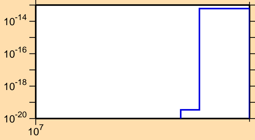
\sigma vs. E for ^{93}\text{Ru}(n,2n\alpha)
