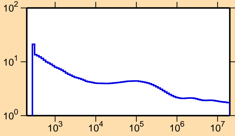
\sigma vs. E for ^{93}\text{Ru}(n,\text{nonel.})
