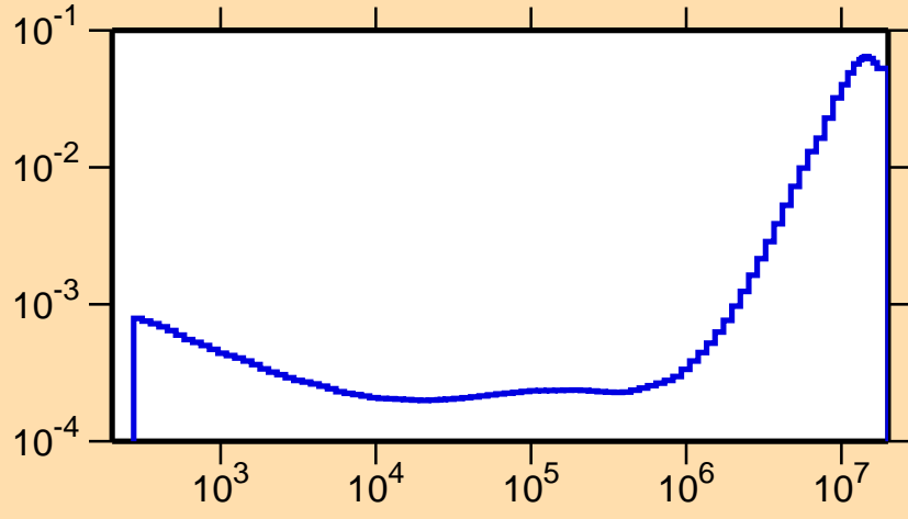
\sigma vs. E for ^{93}\text{Ru}(n,\alpha)
