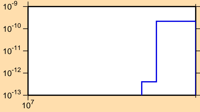
\sigma vs. E for ^{93}\text{Ru} (mt 34)
