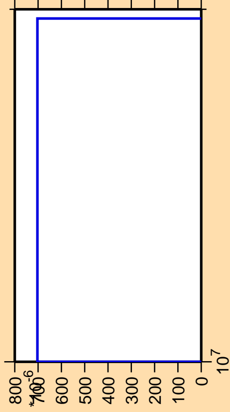
\Delta\sigma/\sigma vs. E for ^{93}\text{Ru}(n,2n\alpha)
