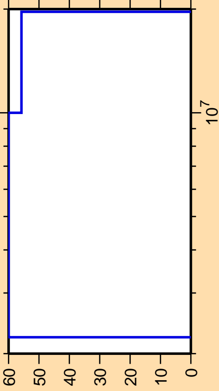
\Delta\sigma/\sigma vs. E for ^{93}\text{Ru}(n,n\text{cont.})
