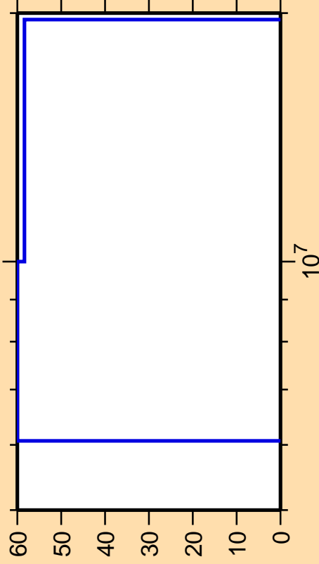
\Delta\sigma/\sigma vs. E for ^{93}\text{Ru}(n,n\alpha)
