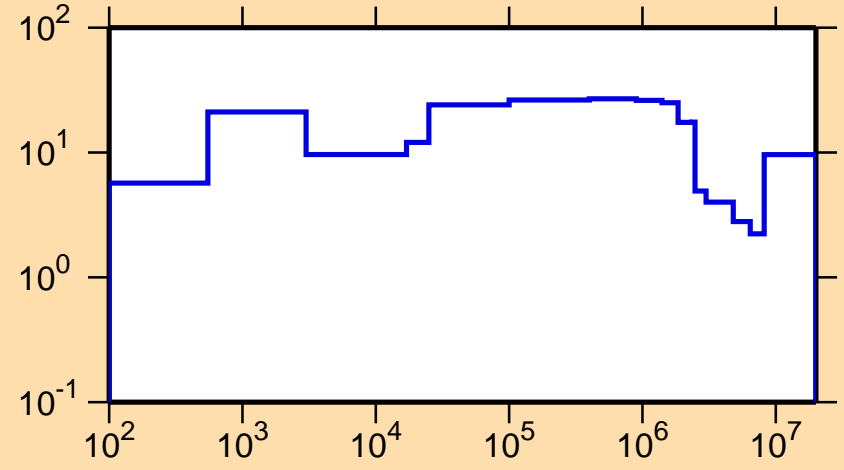
\Delta\sigma/\sigma vs. E for ^{93}\text{Ru}(n,\text{tot.})
