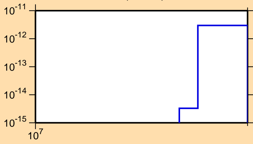
\sigma vs. E for ^{93}\text{Ru}(n,2n\alpha)
