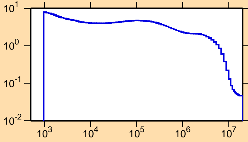
\sigma vs. E for ^{93}\text{Ru}(n,p)
