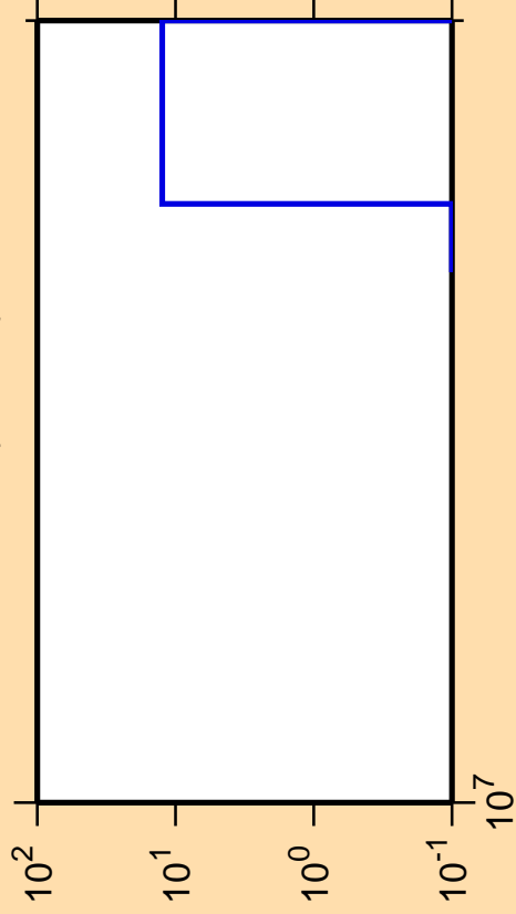
\Delta\sigma/\sigma vs. E for ^{93}\text{Ru}(n,2n\alpha)
