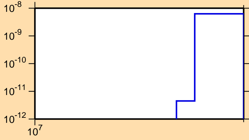
\sigma vs. E for ^{93}\text{Ru} (mt 45)
