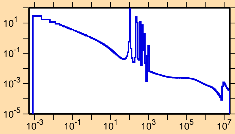
\sigma vs. E for ^{93}\text{Ru}(n,\gamma)
