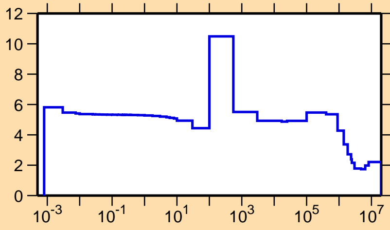
\sigma vs. E for ^{93}\text{Ru}(n,\text{el.})
