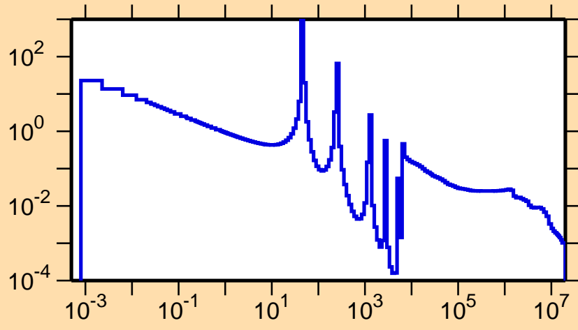
\sigma vs. E for ^{94}\text{Ru}(n,\gamma)
