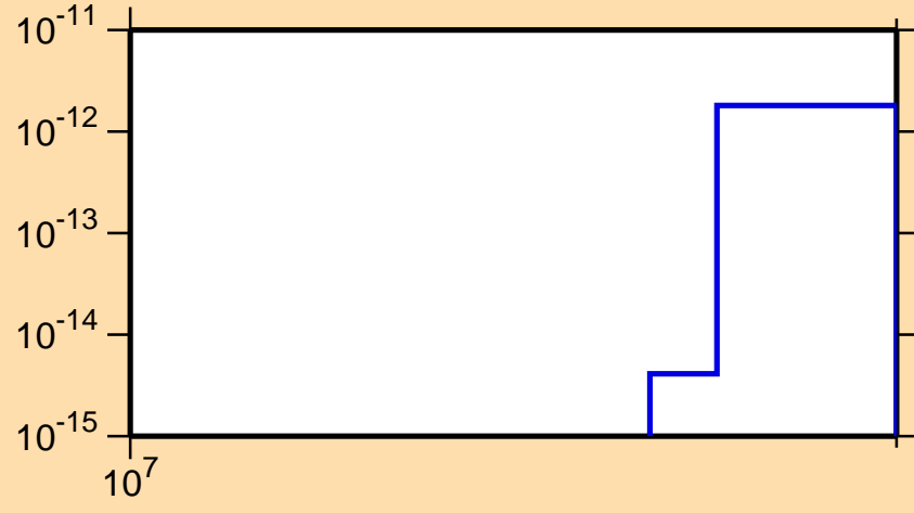
\sigma vs. E for ^{94}\text{Ru}(\text{mt117})
