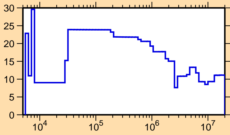
\Delta\sigma/\sigma vs. E for ^{94}\text{Ru}(n,\text{el.})
