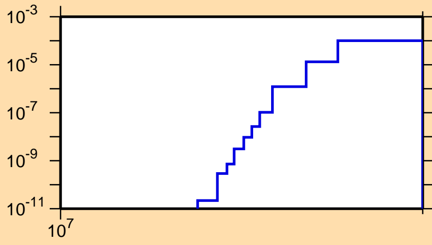
\sigma vs. E for ^{94}\text{Ru}(n,t)
