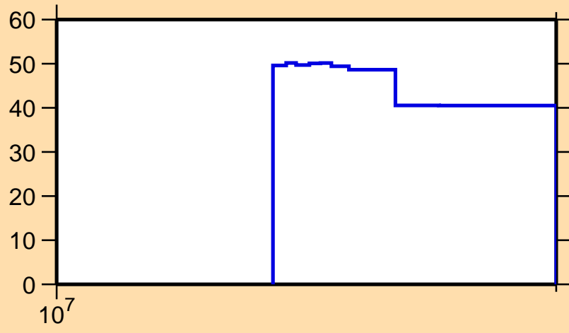
\Delta\sigma/\sigma vs. E for ^{94}\text{Ru}(n,\text{inel.})
