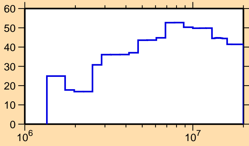
\Delta\sigma/\sigma vs. E for ^{94}\text{Ru}(n,n_1)
