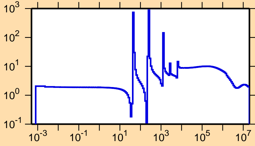
\sigma vs. E for ^{94}\text{Ru}(n,\text{el.})
