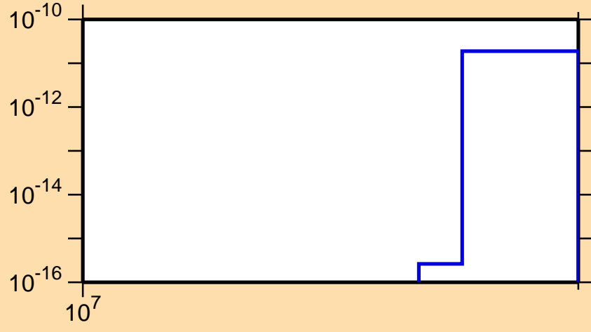
\sigma vs. E for ^{94}\text{Ru}(n,\text{pt})
