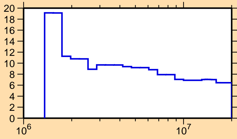
\Delta\sigma/\sigma vs. E for ^{94}\text{Ru}(n,\text{nonel.})
