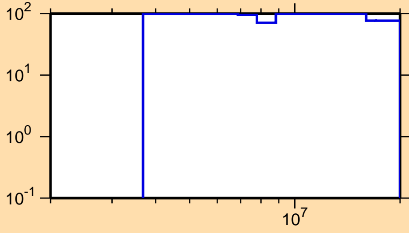
\Delta\sigma/\sigma vs. E for ^{94}\text{Ru}(n,n\text{cont.})
