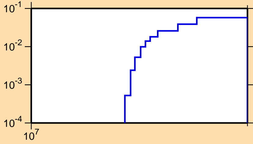
\sigma vs. E for ^{94}\text{Ru}(n,2n)
