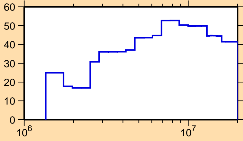
\Delta\sigma/\sigma vs. E for ^{94}\text{Ru}(n,n_1)
