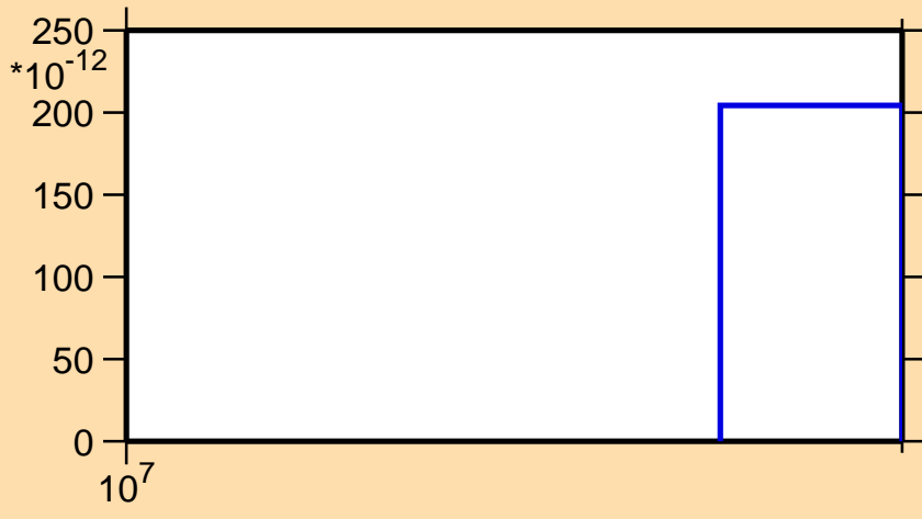
\sigma vs. E for ^{94}\text{Ru}(n,\text{nd})
