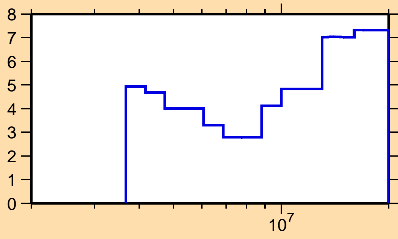
\Delta\sigma/\sigma vs. E for ^{94}\text{Ru}(n,\text{tot.})
