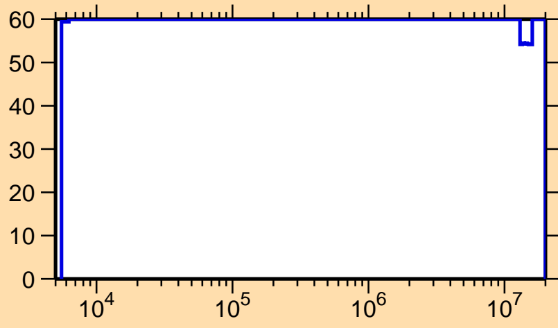
\Delta\sigma/\sigma vs. E for ^{94}\text{Ru}(n,\gamma)
