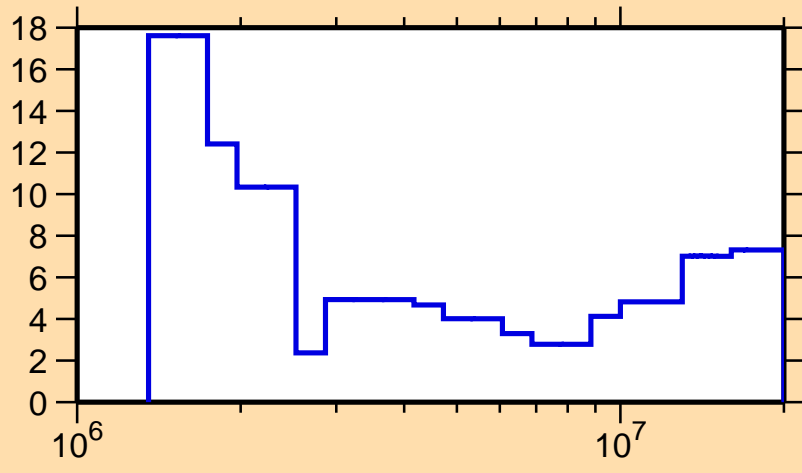
\Delta\sigma/\sigma vs. E for ^{94}\text{Ru}(n,\text{tot.})
