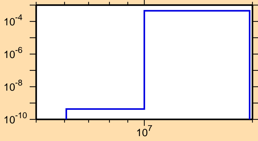
\sigma vs. E for ^{94}\text{Ru}(n,n\alpha)
