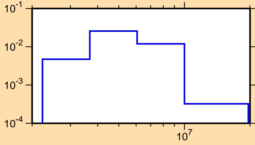
\sigma vs. E for ^{94}\text{Ru}(n,n_3)
