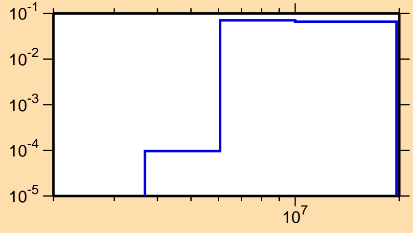
\sigma vs. E for ^{94}\text{Ru}(n,n\text{cont.})
