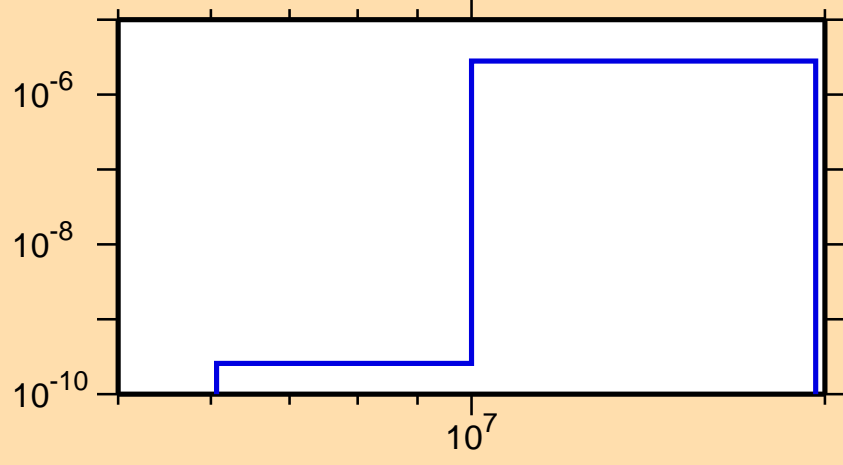
\sigma vs. E for ^{94}\text{Ru}(n,\text{He3})
