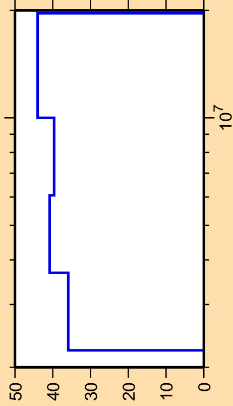
\Delta\sigma/\sigma vs. E for ^{94}\text{Ru}(n,n_3)
