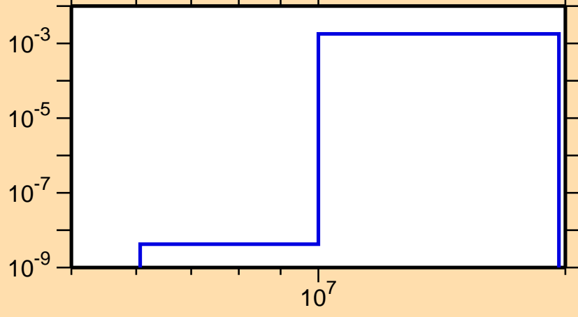
\sigma vs. E for ^{94}\text{Ru}(n,p\alpha)
