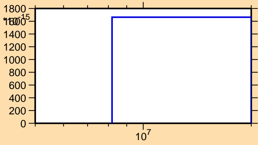
\sigma vs. E for ^{94}\text{Ru}(n,nd)
