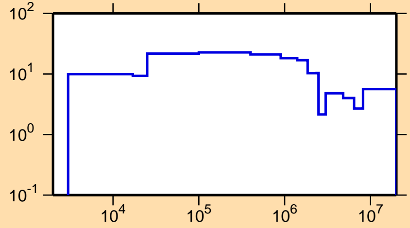
\Delta\sigma/\sigma vs. E for ^{94}\text{Ru}(n,\text{tot.})
