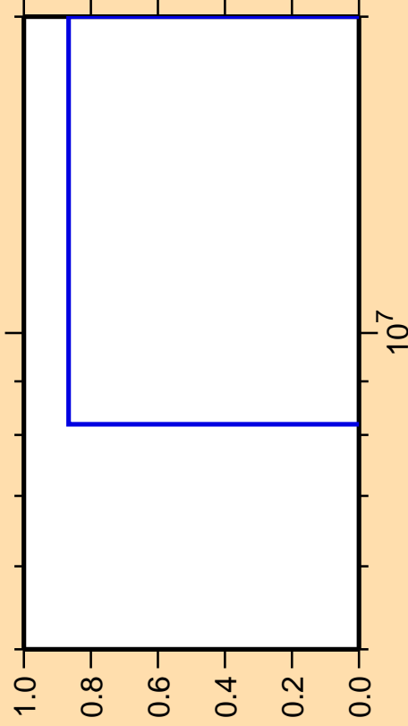
\Delta\sigma/\sigma vs. E for ^{94}\text{Ru}(\text{mt } 45)
