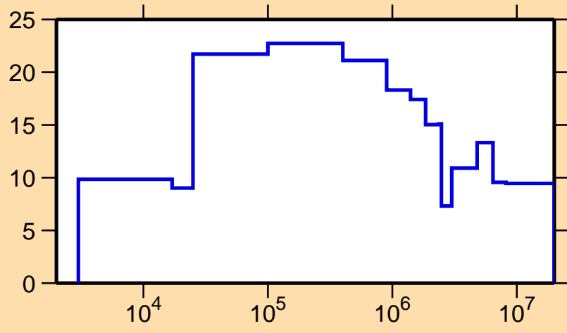
\Delta\sigma/\sigma vs. E for ^{94}\text{Ru}(n,el.)
