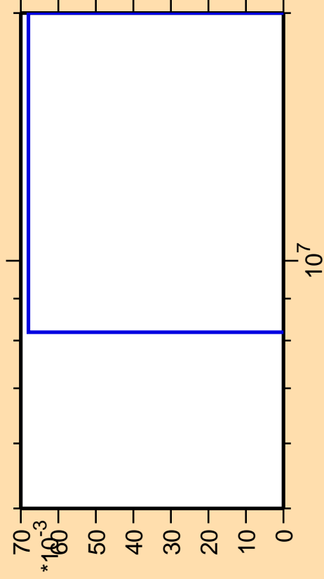
\Delta\sigma/\sigma vs. E for ^{94}\text{Ru}(\text{mt117})
