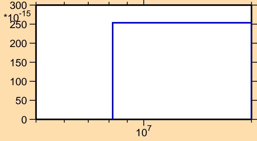
\sigma vs. E for ^{94}\text{Ru}(\text{mt } 45)
