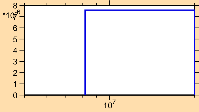
\sigma vs. E for ^{94}\text{Ru}(n,\text{pd})
