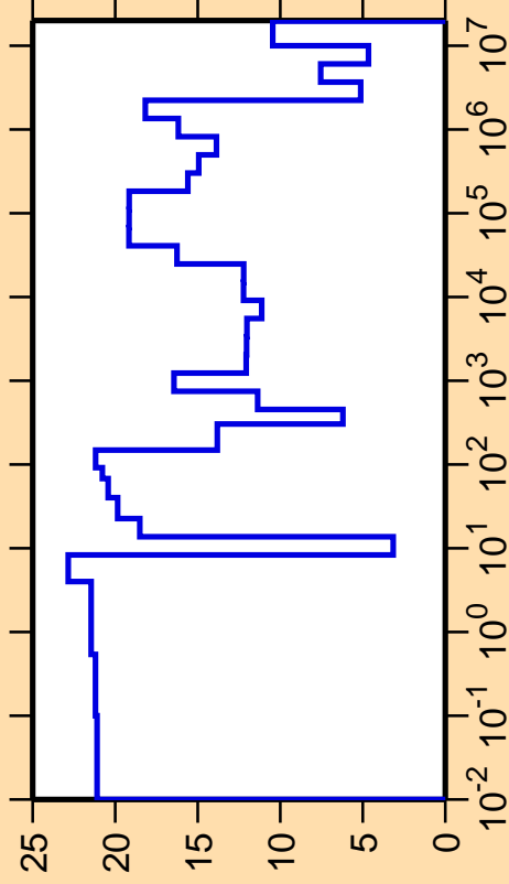
\Delta\sigma/\sigma vs. E for ^{95}\text{Ru}(n,\text{el.})
