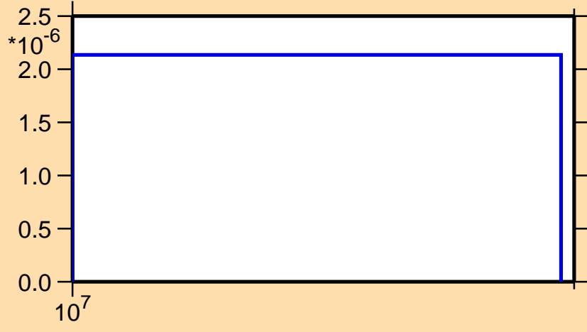
\sigma vs. E for ^{95}\text{Ru}(n,\text{pd})
