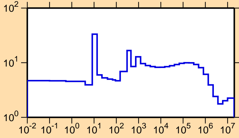
\sigma vs. E for ^{95}\text{Ru}(n,\text{el.})
