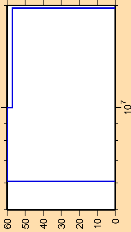
\Delta\sigma/\sigma vs. E for ^{95}\text{Ru}(n,n\alpha)
