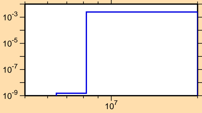
\sigma vs. E for ^{95}\text{Ru}(n,n\alpha)
