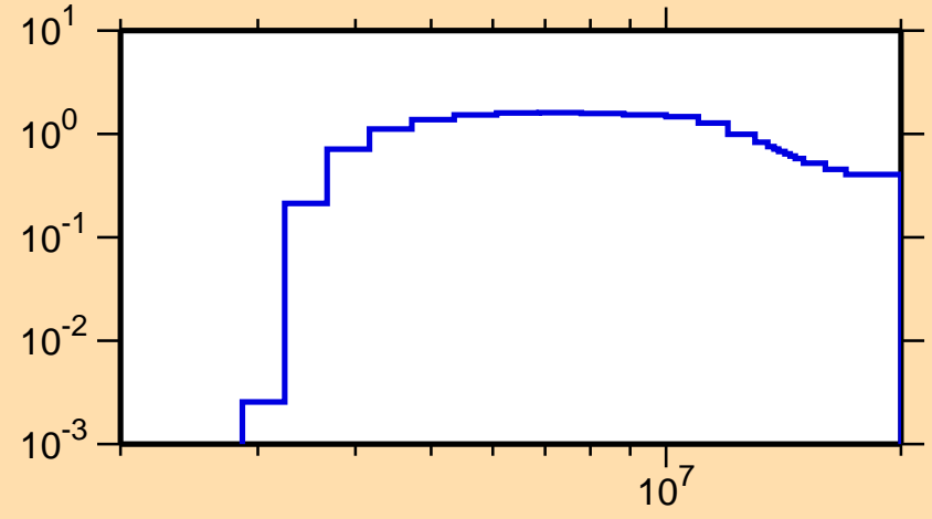
\sigma vs. E for ^{96}\text{Ru}(n,n\text{cont.})
