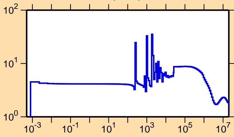
\sigma vs. E for ^{96}\text{Ru}(n,\text{el.})
