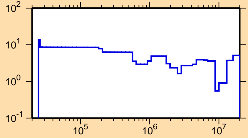
\Delta\sigma/\sigma vs. E for ^{96}\text{Ru}(n,\text{tot.})
