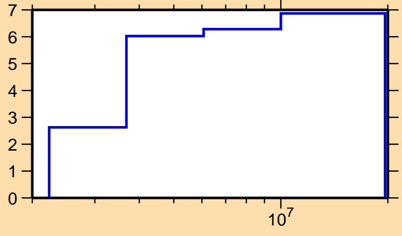
\Delta\sigma/\sigma vs. E for ^{96}\text{Ru}(n,n\text{onel.})
