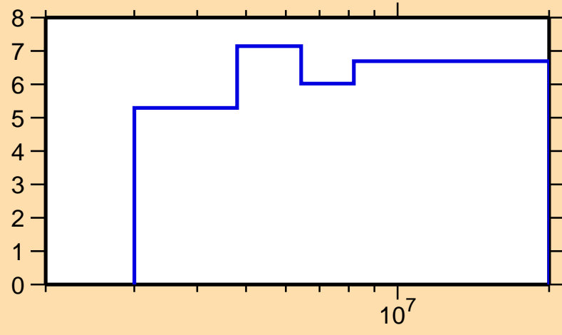
\Delta\sigma/\sigma vs. E for ^{96}\text{Ru}(n,n\text{nonel.})
