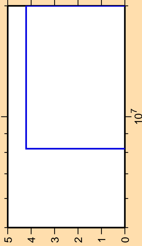
\Delta\sigma/\sigma vs. E for ^{96}\text{Ru}(n,\text{pt})
