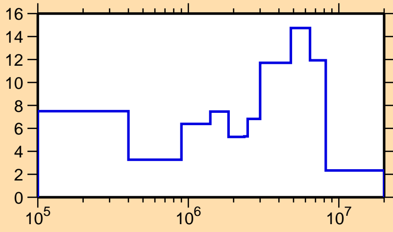
\Delta\sigma/\sigma vs. E for ^{96}\text{Ru}(n,el.)
