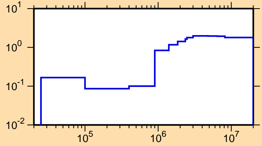
\sigma vs. E for ^{96}\text{Ru}(n,\text{nonel.})
