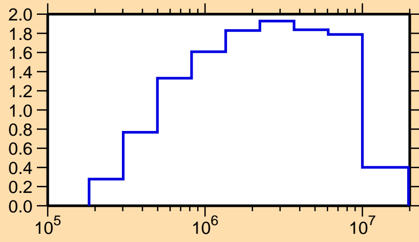
\sigma vs. E for ^{97}\text{Ru}(n,\text{inel.})
