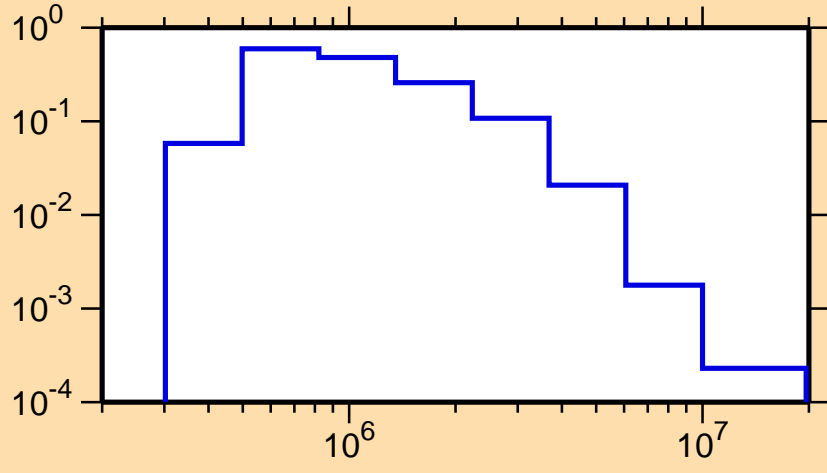
\sigma vs. E for ^{97}\text{Ru}(n,n_2)
