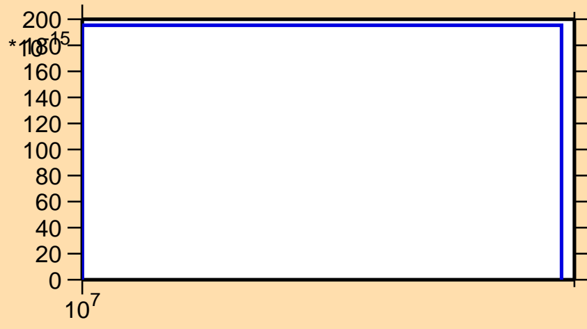
\sigma vs. E for ^{97}\text{Ru} (mt 34)
