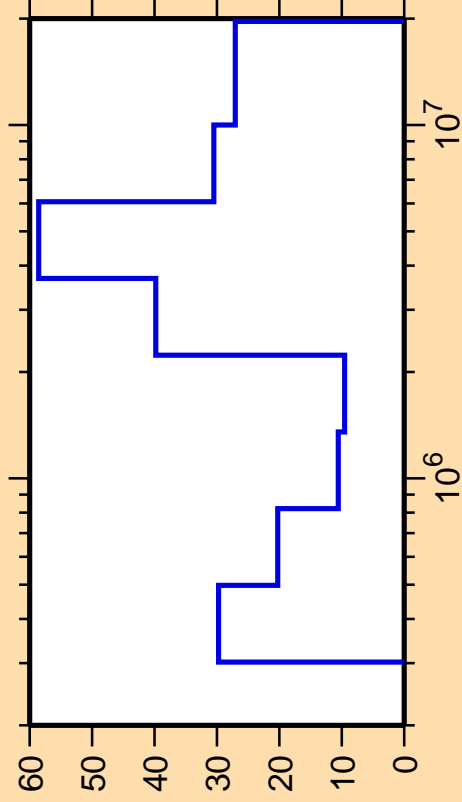
\Delta\sigma/\sigma vs. E for ^{97}\text{Ru}(n,n_2)
