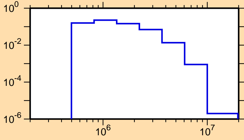
\sigma vs. E for ^{97}\text{Ru}(n,n_3)
