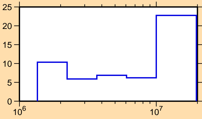
\Delta\sigma/\sigma vs. E for ^{97}\text{Ru}(n,\text{inel.})
