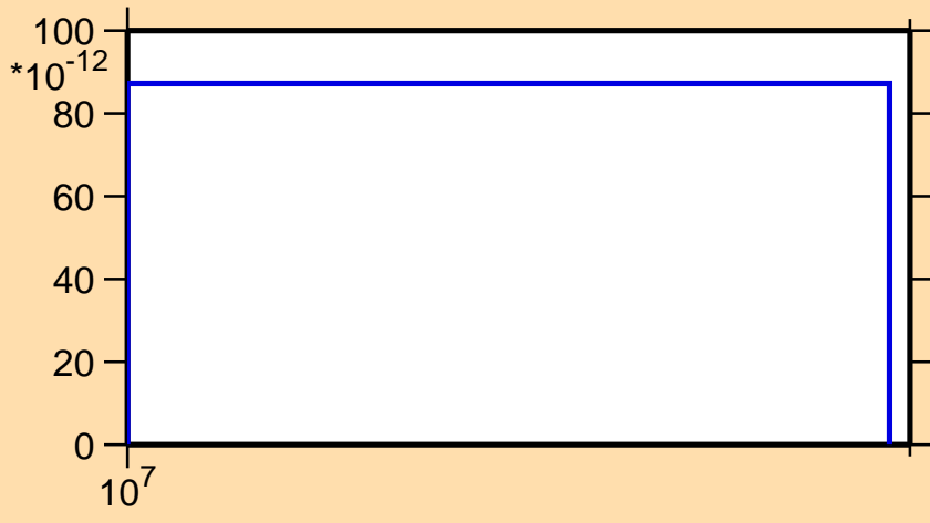
\sigma vs. E for ^{97}\text{Ru}(\text{mt117})
