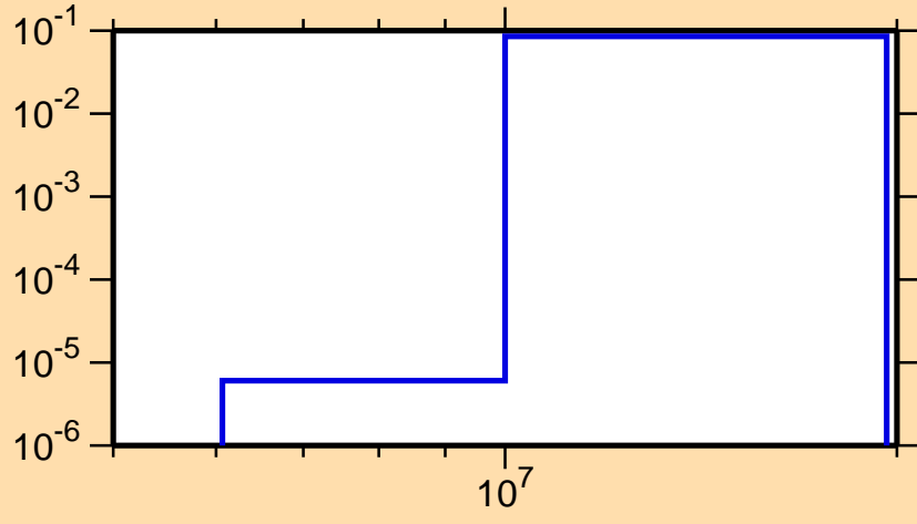
\sigma vs. E for ^{97}\text{Ru}(n,np)
