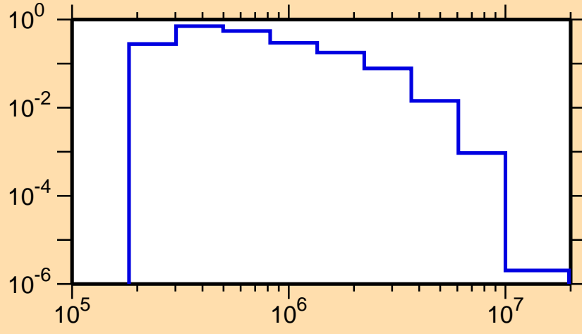
\sigma vs. E for ^{97}\text{Ru}(n,n_1)
