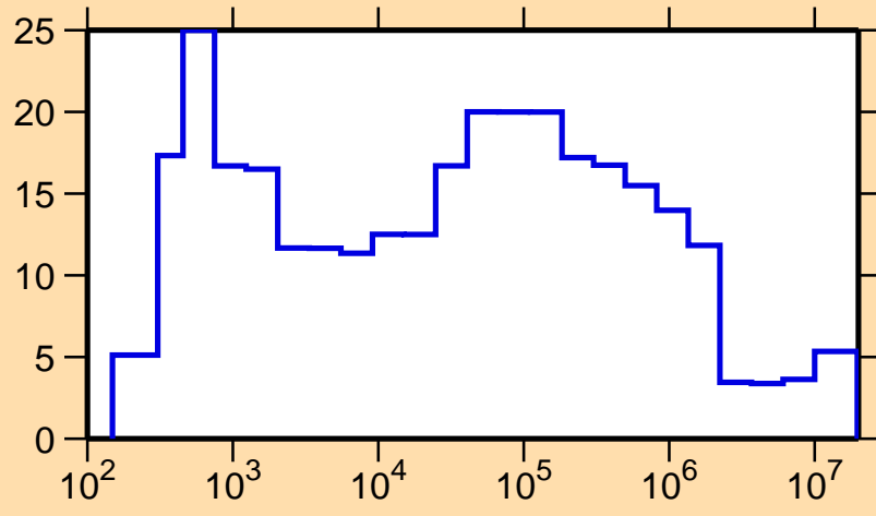
\Delta\sigma/\sigma vs. E for ^{97}\text{Ru}(n,\text{tot.})
