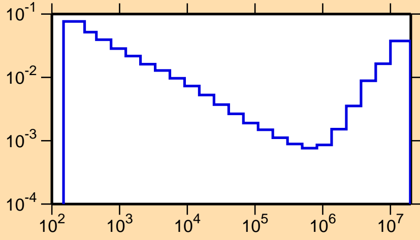
\sigma vs. E for ^{97}\text{Ru}(n,\alpha)
