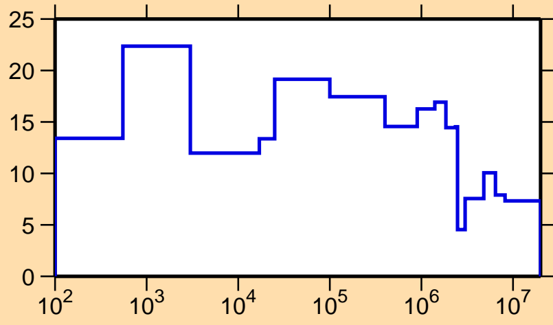
\Delta\sigma/\sigma vs. E for ^{97}\text{Ru}(n,el.)
