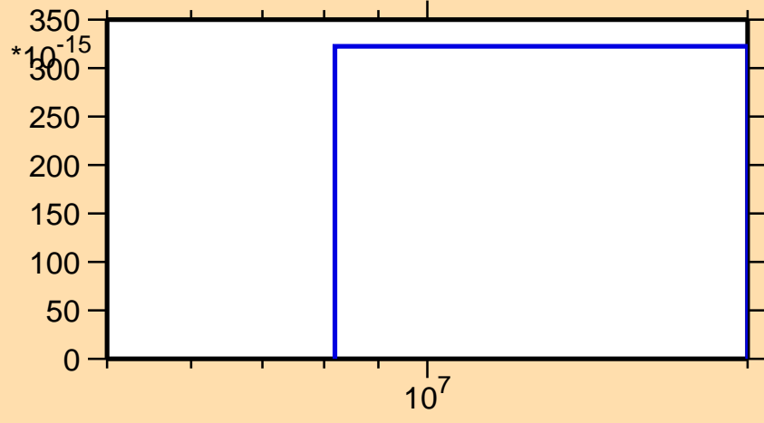
\sigma vs. E for ^{98}\text{Ru}(\text{mt } 45)
