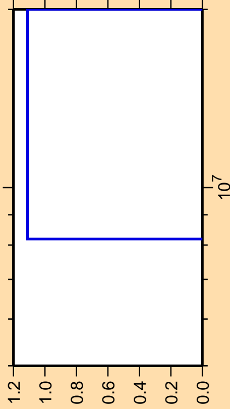
\Delta\sigma/\sigma vs. E for ^{98}\text{Ru}(\text{mt } 45)
