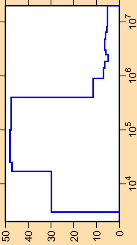
\Delta\sigma/\sigma vs. E for ^{98}\text{Ru}(n,\text{nonel.})
