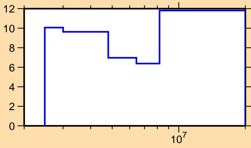
\Delta\sigma/\sigma vs. E for ^{98}\text{Ru}(n,ncont.)
