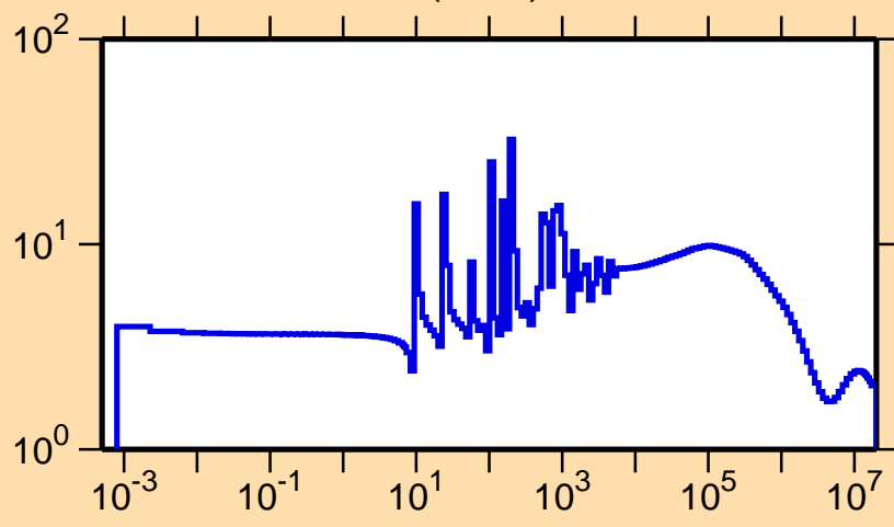
\sigma vs. E for ^{99}\text{Ru}(n,\text{el.})
