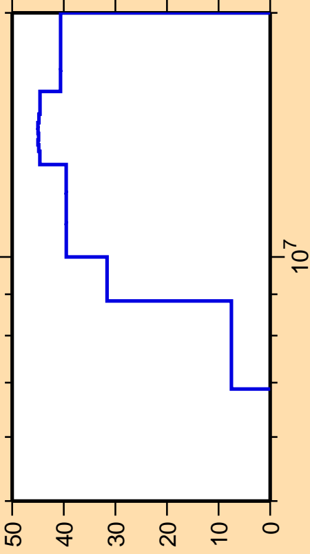
\Delta\sigma/\sigma vs. E for ^{99}\text{Ru}(n,n\text{cont.})
