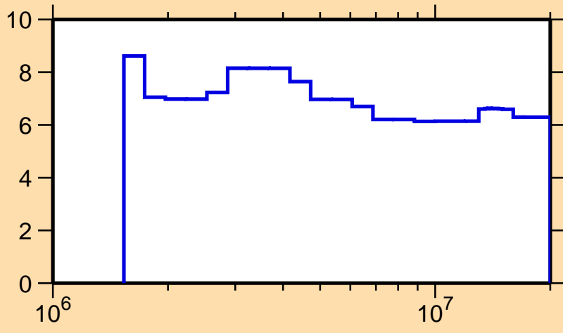
\Delta\sigma/\sigma vs. E for ^{99}\text{Ru}(n,n\text{nonel.})
