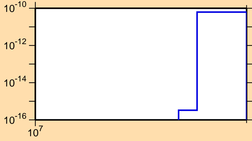
\sigma vs. E for ^{99}\text{Ru}(n,pt)
