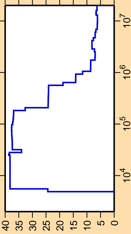
\Delta\sigma/\sigma vs. E for ^{99}\text{Ru}(n,\text{nonel.})
