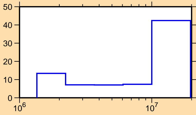
\Delta\sigma/\sigma vs. E for ^{99}\text{Ru}(n,ncont.)
