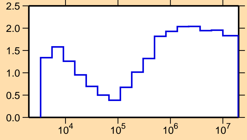
\sigma vs. E for ^{99}\text{Ru}(n,\text{nonel.})
