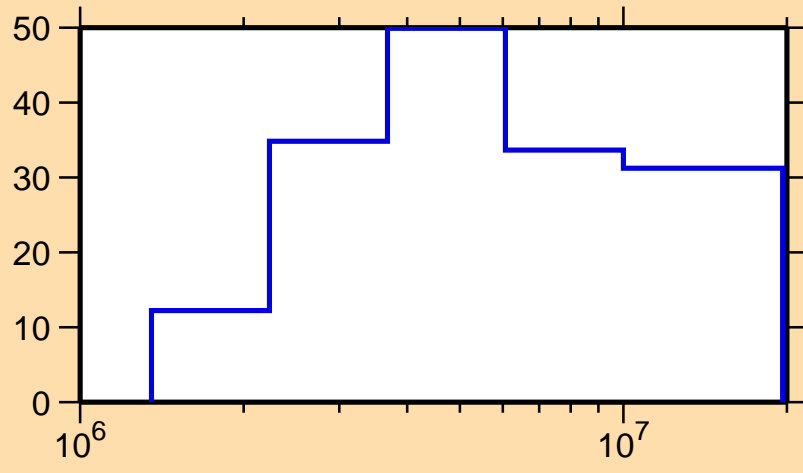
\Delta\sigma/\sigma vs. E for ^{99}\text{Ru}(n,n_1)
