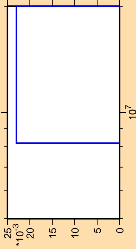
\Delta\sigma/\sigma vs. E for ^{99}\text{Ru}(\text{mt } 34)
