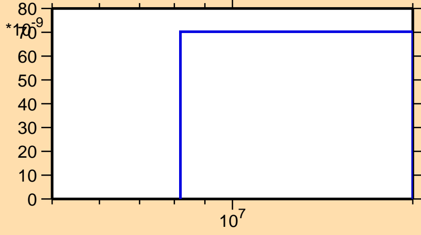
\sigma vs. E for ^{99}\text{Ru}(n,p\alpha)
