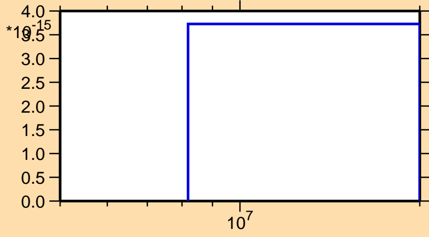
\sigma vs. E for ^{99}\text{Ru}(\text{mt } 34)
