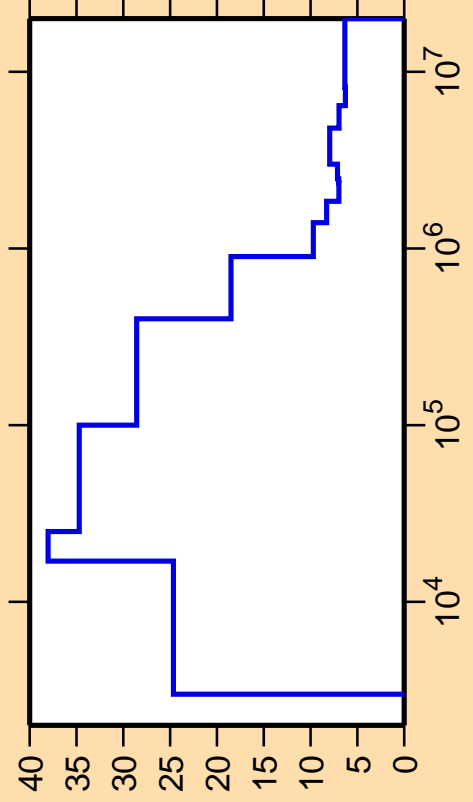
\Delta\sigma/\sigma vs. E for ^{99}\text{Ru}(n,\text{nonel.})
