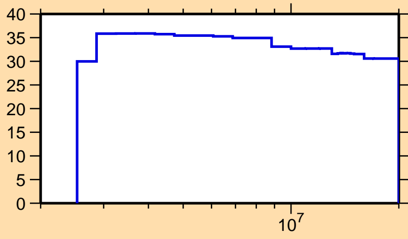
\Delta\sigma/\sigma vs. E for ^{100}\text{Ru}(n,n_1)
