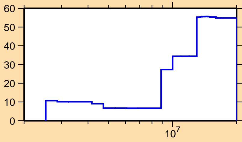
\Delta\sigma/\sigma vs. E for ^{100}\text{Ru}(n,n\text{cont.})
