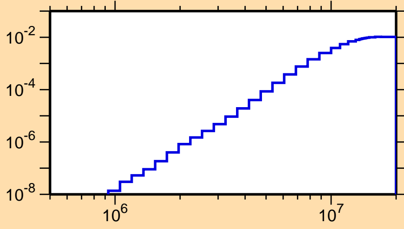
\sigma vs. E for ^{100}\text{Ru}(n,\alpha)
