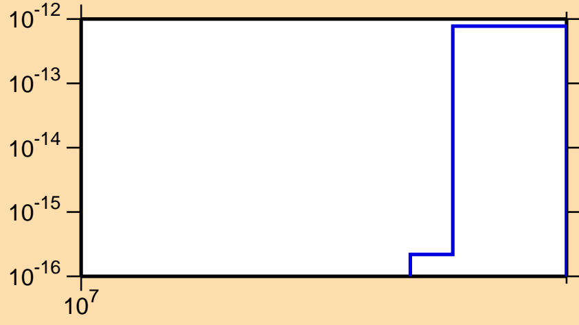
\sigma vs. E for ^{100}\text{Ru}(\text{mt117})
